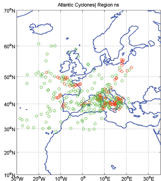
Fig. 4. Spatial distribution of positions of depression centres associated with “intense” precipitation occurred over the NS region. Red (Green) circles denote a SLOW (NON-SLOW) speed of the depression centre during the preceding 6 h.
