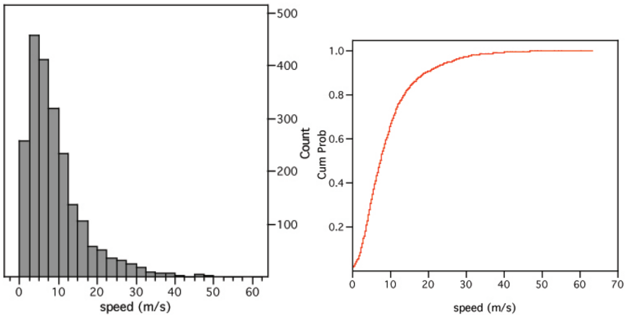
Fig. 3. Histogram and cumulative distribution function of the number of depressions centres (over all the 5 regions in which Italy was divided) with respect to their speed.
