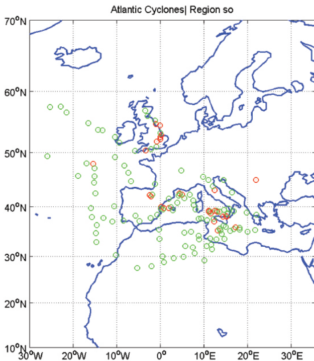
Fig. 5. As Fig. 4, but for the South (SO) region.
