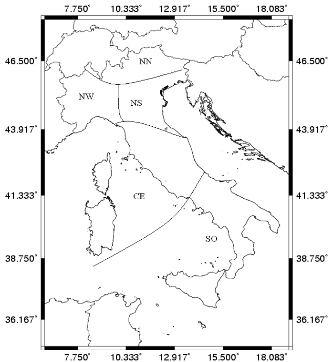
Fig. 1. Division of Italy in the five precipitation climatological regions as obtained by PCA analysis by Brunetti et al. (2004). (Adapted from Brunetti et al., 2004).
