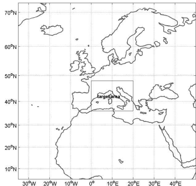
Fig. 2. The domain used for tracking the centres of depressions associated with “intense” precipitation over Italy. The rectangle within the domain is the area where a relationship between SLOW speeds of depression centre and “intense” precipitation over Italy is searched for.
