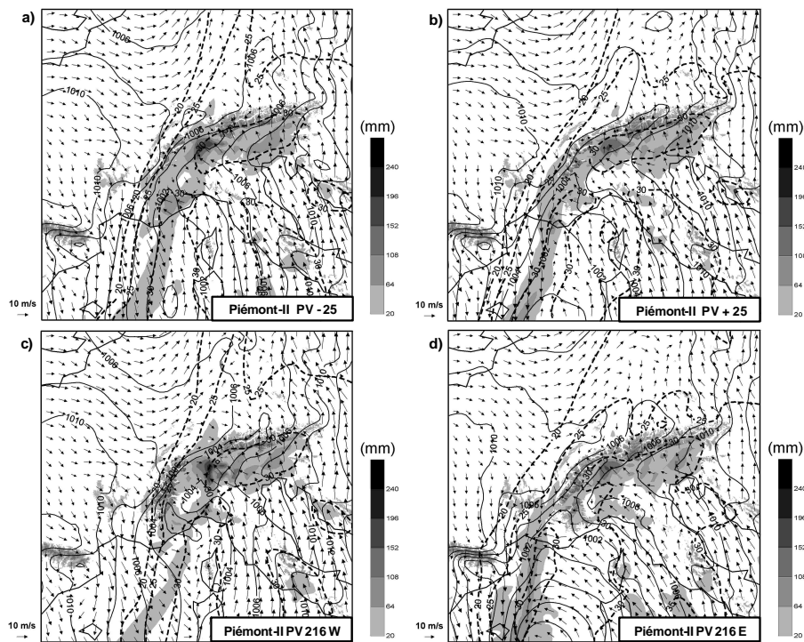
Fig. 17. Perturbed simulations of the Piémont-II event for the fine domain, showing the same fields as in Fig. 8a for the experiments: (a) PV -25 ; (b) PV +25 ; (c) PV 216W; and (d) PV 216E. Maximum precipitation value in (a), (b), (c) and (d) is 196, 205, 240 and 177 mm, respectively.
