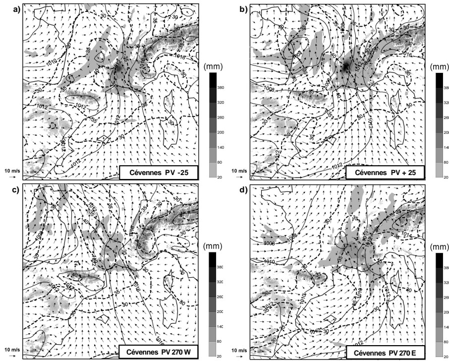
Fig. 13. Perturbed simulations of the Cévennes event for the fine domain, showing the same fields as in Fig. 4a for the experiments: (a) PV -25 ; (b) PV +25 ; (c) PV 270W; and (d) PV 270E. Maximum precipitation value in (a), (b), (c) and (d) is 309, 438, 211 and 183 mm, respectively.
