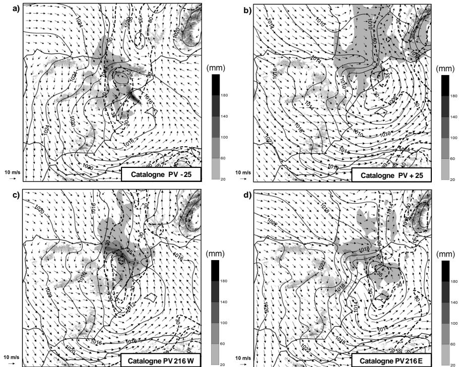
Fig. 11. Perturbed simulations of the Catalogne event for the fine domain, showing the same fields as in Fig. 2a for the experiments: (a) PV -25 ; (b) PV +25 ; (c) PV 216W; and (d) PV 216E. Maximum precipitation value in (a), (b), (c) and (d) is 230, 91, 157 and 79 mm, respectively.
