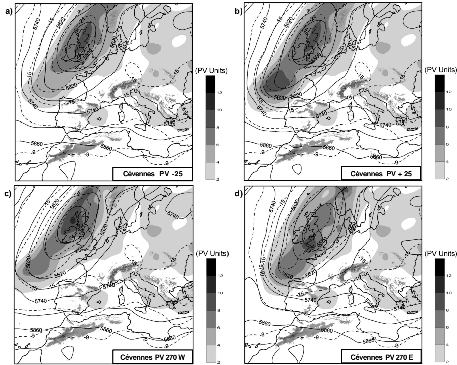
Fig. 12. Perturbed simulations of the Cévennes event for the coarse domain, showing the same fields as in Fig. 3a for the experiments: (a) PV -25 ; (b) PV +25 ; (c) PV 270W; and (d) PV 270E.
