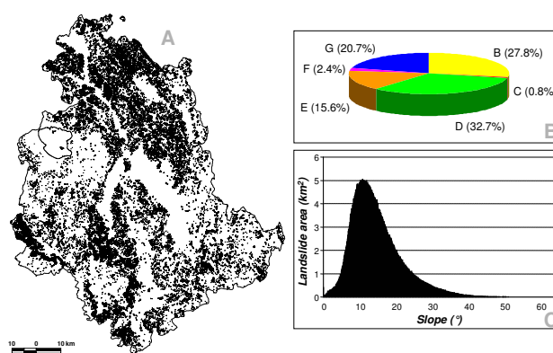
Fig. 4. Geomorphological landslide inventory map. A) Geographical distribution of landslides. B) Abundance of landslide areas in the rock units cropping out in the Region (for colour legend see Fig. 1). C) Landslide abundance and terrain gradient.
