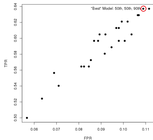
Figure 8. The moderate-hazard nowcast was calibrated by calculating r_j , the distance to perfect classification, for a variety of rainfall and ARI thresholds that ranged from the 50th to the 95th percentile values. The lowest (best) r_j value was observed for the 50th percentile ARI, 50th percentile rainfall over moist-condition ground and 90th percentile rainfall over dry-condition ground. These thresholds are represented by the second dot from the right in the red circle. Ideally, the choice of the “best” rainfall thresholds depends upon the intended use of the model and the economic costs of different errors. Since these details are not yet available, r_j was selected to provide a balanced and easily interpreted measure of model success.
