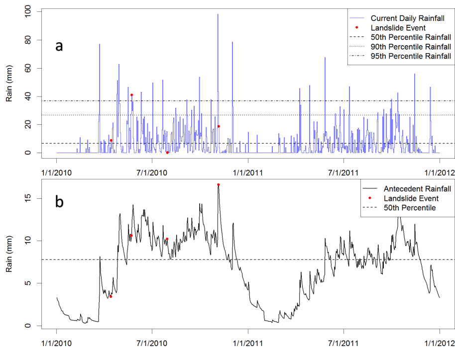
Figure 7. Example time series of (a) rainfall and (b) antecedent rainfall for a pixel west of San Jose, Costa Rica. The time series highlight four landslides that were reported in this area in 2010: 14 April, 22 May, 30 July and 5 November (shown as red circles). The first landslide (Fig. 9a) occurred very early in the year before the peak rainy season and a nowcast was not issued. The time series shown in the upper graph indicates that a moderate-hazard nowcast was triggered for the 5 November event and a high-hazard nowcast was triggered for the 22 May event (Fig. 9b). However, due to the antecedent rainfall for the 14 April event and low rainfall totals for the 30 July event, no nowcasts were issued.
