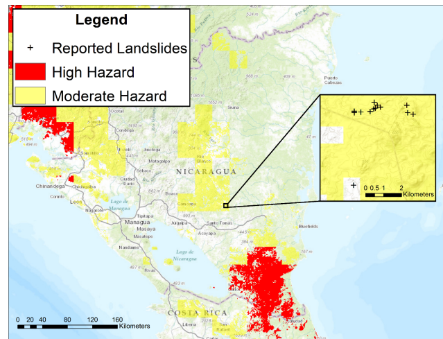
Figure 10. Landslide hazard potential for 23 June 2014. Black crosses indicate locations where a cluster of landslides occurred near El Ayote, Nicaragua. Yellow pixels (moderate hazard) and red pixels (high hazard) are shown for that day. Of 14 landslides, 13 were predicted by the moderate-hazard category. The southernmost landslide was located in a relatively flat location that had been mapped as having “very low” landslide susceptibility, so it was not predicted despite daily rainfall exceeding the 50th percentile threshold.
