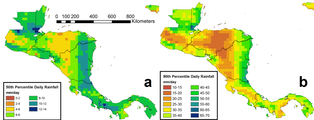
Figure 3. Maps showing rainfall values in \text{mm day}^{-1} for (a) 50th and (b) 90th percentiles calculated from TMPA daily rainfall estimates covering the years 2001–2013. These two percentile maps were used within the decision tree framework to produce moderate landslide hazard nowcasts.
