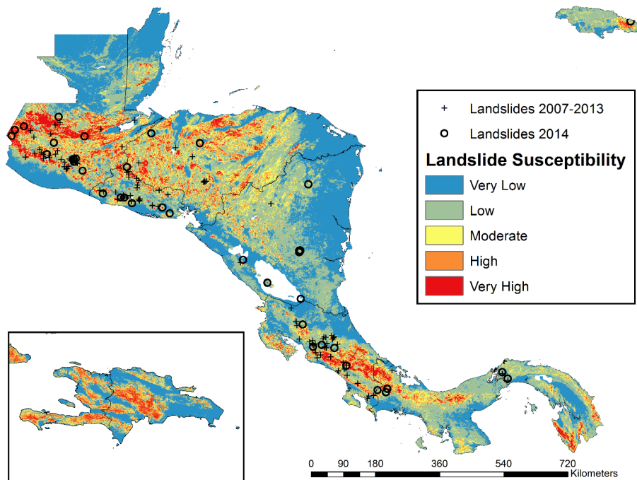
Figure 1. Regional landslide susceptibility map created using a fuzzy overlay methodology from global slope, soil and road databases as well as a regional map of faults at a resolution of 30 arcsec (approximately 1 km) (Kirschbaum et al., 2015a). Landslides recorded in the study areas are shown for the years 2007–2013 (+) and 2014 (o). Overall, 166 landslide reports are from the Global Landslide Catalog and 24 landslides in El Salvador were selected from the MARN catalog. Large numbers of landslides are located near capital cities, implying some degree of reporting bias. Inset map shows landslide susceptibility map for Hispaniola with 31 reported landslides.
