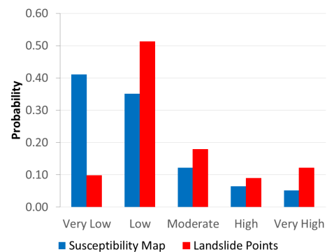
Figure 2. Probability distribution of susceptibility values at landslide locations reported from 2007 to 2013 compared to landslide susceptibility values for all of Central America. Landslides occurred in all susceptibility categories, but few landslides (< 10 %) occurred in the lowest category. The LHASA model used a threshold of “low” susceptibility or greater ( SI \geq 2 ) with rainfall and antecedent rainfall thresholds within the decision tree framework (Fig. 6). SI \geq 2 (low) was chosen to exclude a large portion of Central America without losing the ability to predict most landslide events.
