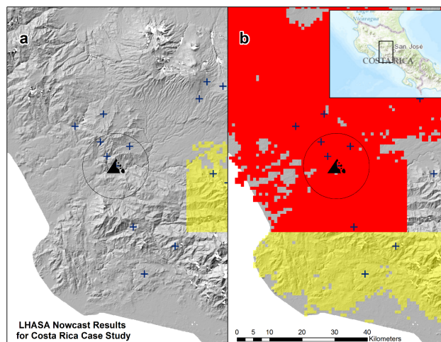
Figure 9. This shows the results of the model nowcasts for a cluster of rockfalls (denoted by a single black rockfall icon) that occurred within the same area of the highway near Orotina, Costa Rica, for two dates in 2010: (a) 14 April and (b) 22 May. The black circle indicates the estimated maximum spatial error of these landslide reports (10 km), suggesting that the landslides could have occurred anywhere within that area. Blue crosses indicate the locations of other landslides in the GLC from 2007 to 2013. The 14 April event did not generate a moderate-hazard nowcast (yellow), but enough rainfall was observed to the east of the landslide location to trigger a moderate-hazard nowcast. Comparatively, the 22 May event (b) shows that many high- and moderate-hazard nowcasts were generated within the proximity of the reported event.
