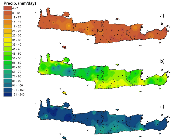
Figure 2. Spatially interpolated (IDW) daily precipitation fields for the (a) 50th percentile, (b) 95th percentile and (c) 99.5th percentile, based on records from 69 gauging stations.
