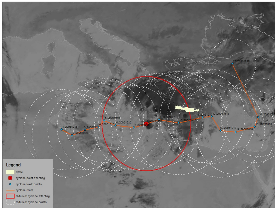
Figure 3. The track and radius of each track point of the cyclone which caused the flash flood in Almirida on 17 October 2006. The background information is the infrared METEOSAT image at 00:00 UTC on 17 October 2006.
