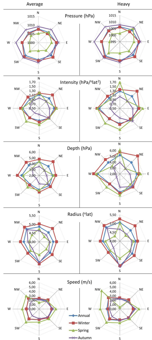
Figure 8. Seasonal and annual analysis of the basic characteristics of the cyclones triggering precipitation events over Crete island for the period 1979–2011. The left column represents the average for all rain events and the right column only represents heavy precipitation events.
