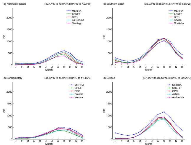
Figure 5. Monthly mean DC for four regions in southern Europe. MERRA, SHEFF and CPC DC are from the GFWD gridded fields over the latitude and longitude range specified in the caption. The other two DC plots are for representative weather stations in that range.
