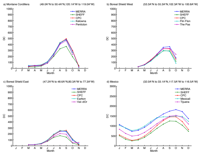
Figure 2. Monthly mean Drought Code (DC) for three regions in Canada and northwestern Mexico. MERRA, SHEFF and CPC DC are from the GFWED gridded fields over the latitude and longitude range specified in the caption. The other two DC plots are for representative weather stations in that range. Note the different DC scale for Mexico.
