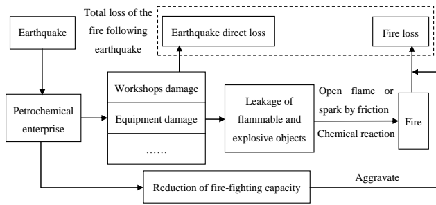
Fig. 1. Post-earthquake fire-causing mechanism of the petrochemical enterprises.
