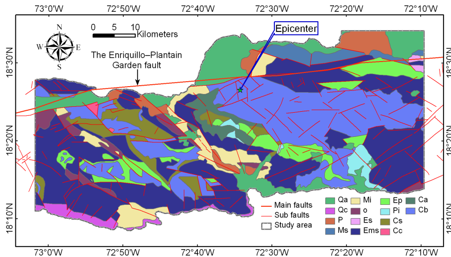
Figure 2. The bedrock distribution map of the study area.
