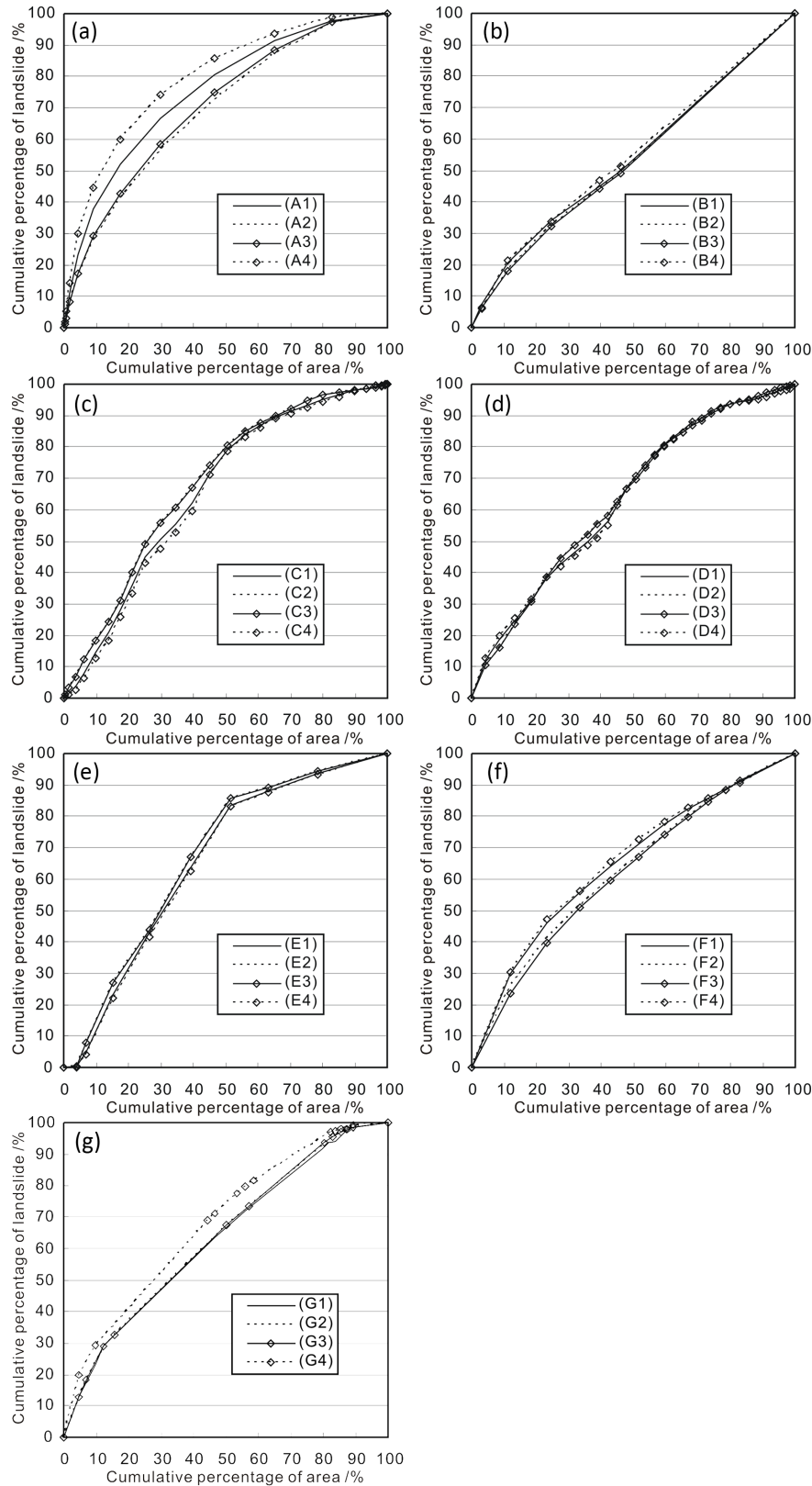
Figure 26. Cumulative landslide area curves to analyze the influence of the seven impact parameters on the landslide occurrences, separately shown by different impact parameters. A: slope angle, B: slope curvature, C: distance from epicenter, D: distance from the Enriquillo–Plantain Garden fault, E: PGA, F: distance from drainages, and G: lithology. The curves are: 1: landslide area, 2: landslide centroid point number, 3: ;and slide top point number, and 4: landslide accumulation material volume.
