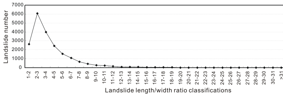
Figure 14. Landslide length/width ratio distribution.
