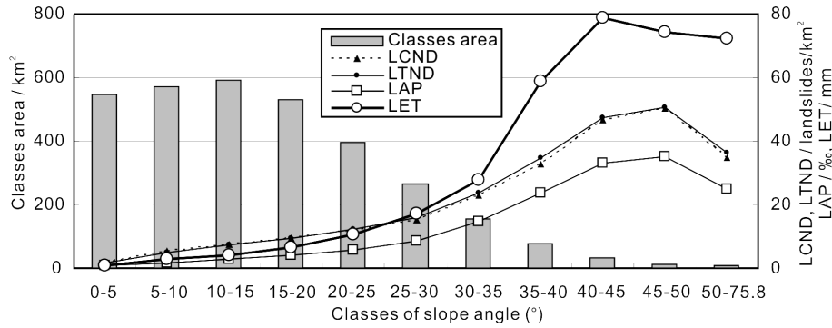
Figure 18. Relationships of co-seismic landslide abundances with slope angles.
