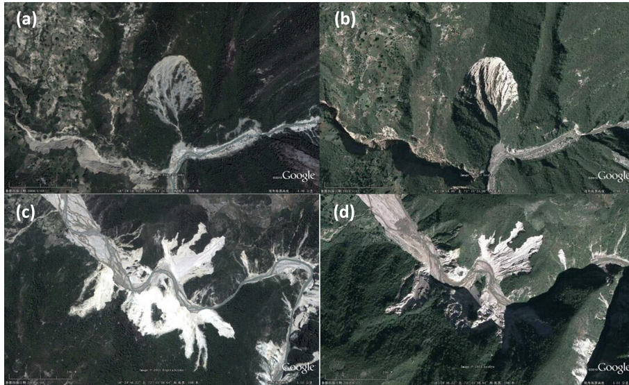
Figure 3. Pre-earthquake landslides are shown in two locations. (a) and (b) are located at 18^{\circ}29'02.70'' N, 72^{\circ}11'22.28'' W; (c) and (d) are located at 18^{\circ}29'46.48'' N, 72^{\circ}11'37.86'' W. (a) and (c) were taken on 10 May 2008 and (b) and (d) were taken on 13 January 2010.
