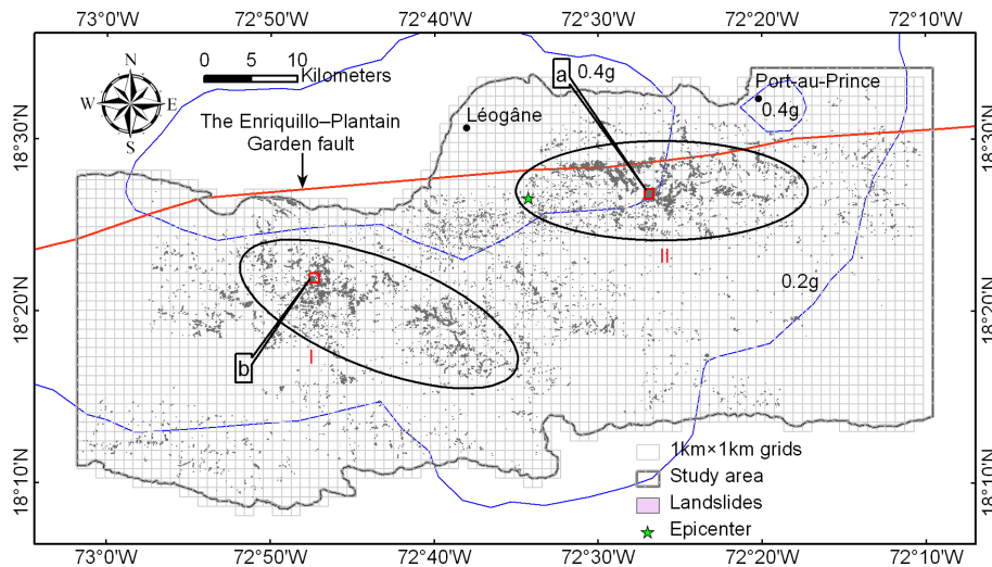
Figure 10. Spatial distribution of landslides triggered by the Haiti earthquake. Blue lines represent PGA contours downloaded from US Geological Survey (2010). I and II are two landslide high density areas. We also constructed 1 km \times 1 km grid cells (shown in gray). The red square (a) represents the grid cell with the highest value of landslide number density and landslide area percentage, and (b) represents the grid cell with the highest value of landslide erosion thickness.
