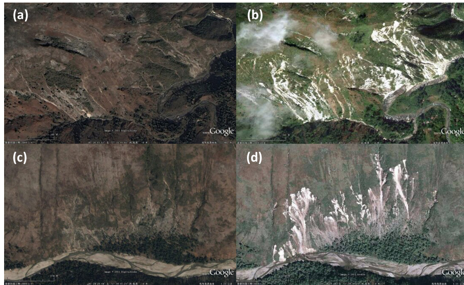
Figure 7. Development of shallow disrupted landslides. The first site is located at 18^{\circ}26'13.52'' N, 72^{\circ}25'44.65'' W as shown in (a) and (b). The dates of the images are 4 February 2009 and 8 November 2010, respectively. The second site (shown in c and d) is located at 18^{\circ}28'29.18'' N, 72^{\circ}30'47.24'' W; they were taken on 4 February 2009 and 13 January 2010, respectively (upwards is north for all four images).
