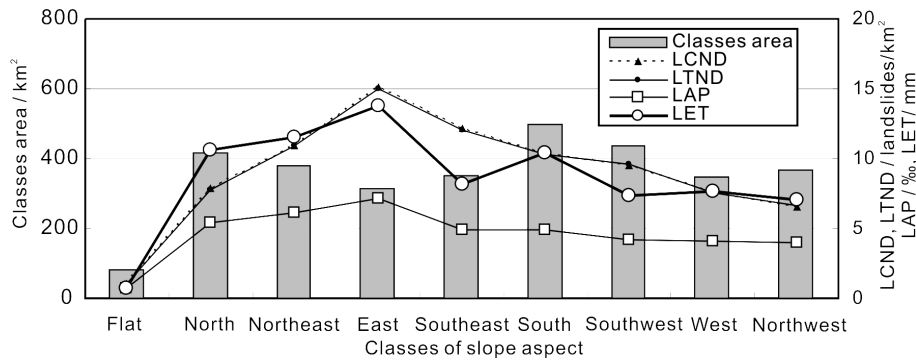
Figure 19. Relationships of co-seismic landslide abundance with slope aspects.
