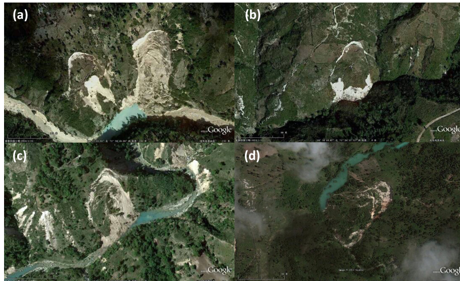
Figure 6. Several typical co-seismic coherent deep-seated landslides. (a) two coherent deep-seated landslides ( 18^{\circ}17'54.15'' N, 72^{\circ}38'18.95'' W) within a short distance; the image is taken on 25 January 2010 (upward is north). (b) is located at 18^{\circ}18'50.87'' N, 72^{\circ}36'57.32'' W, and the image was taken on 25 January 2010 (upward is north). (c) is located at 18^{\circ}19'37.21'' N, 72^{\circ}39'47.57'' W; the image is taken on 25 January 2010 (upward is west). (d) is located at 18^{\circ}12'17.83'' N, 72^{\circ}43'35.27'' W and the image is taken on 27 June 2010 (upward is north).
