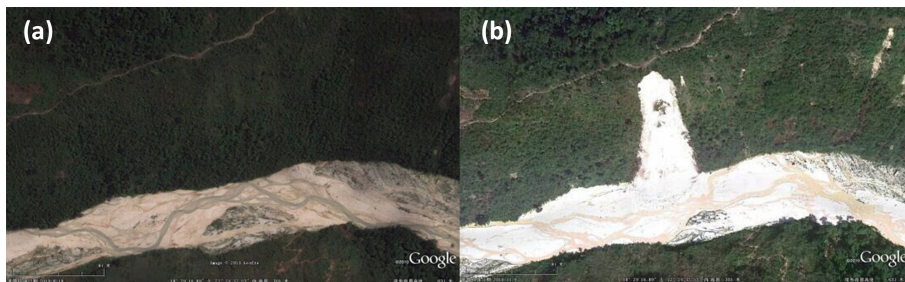
Figure 4. A landslide ( 18^{\circ}29'16.89'' N, 72^{\circ}24'37.53'' W) occurred after the earthquake but may have been triggered by rainfall. (a) was taken on 18 August 2010 and (b) was taken on 9 November 2010 (upward is north).
