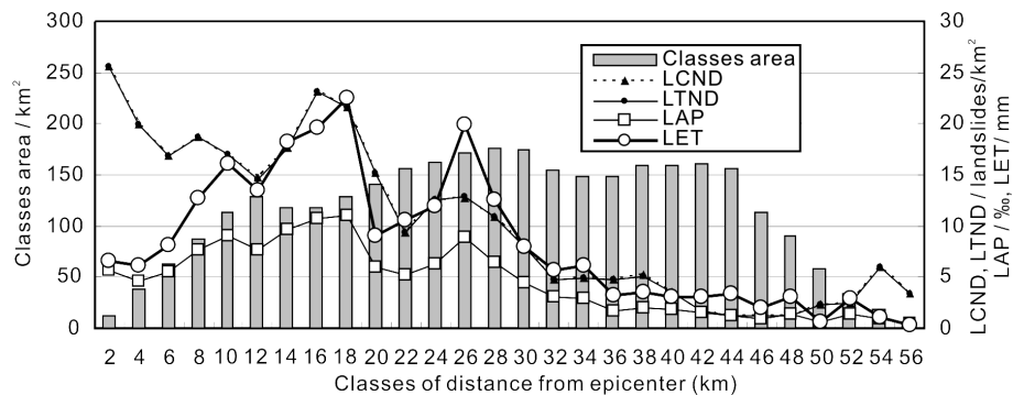
Figure 22. Relationships of co-seismic landslides and distance from epicenter. In all, 28 classes were divided according to 2 km intervals from the epicenter.
