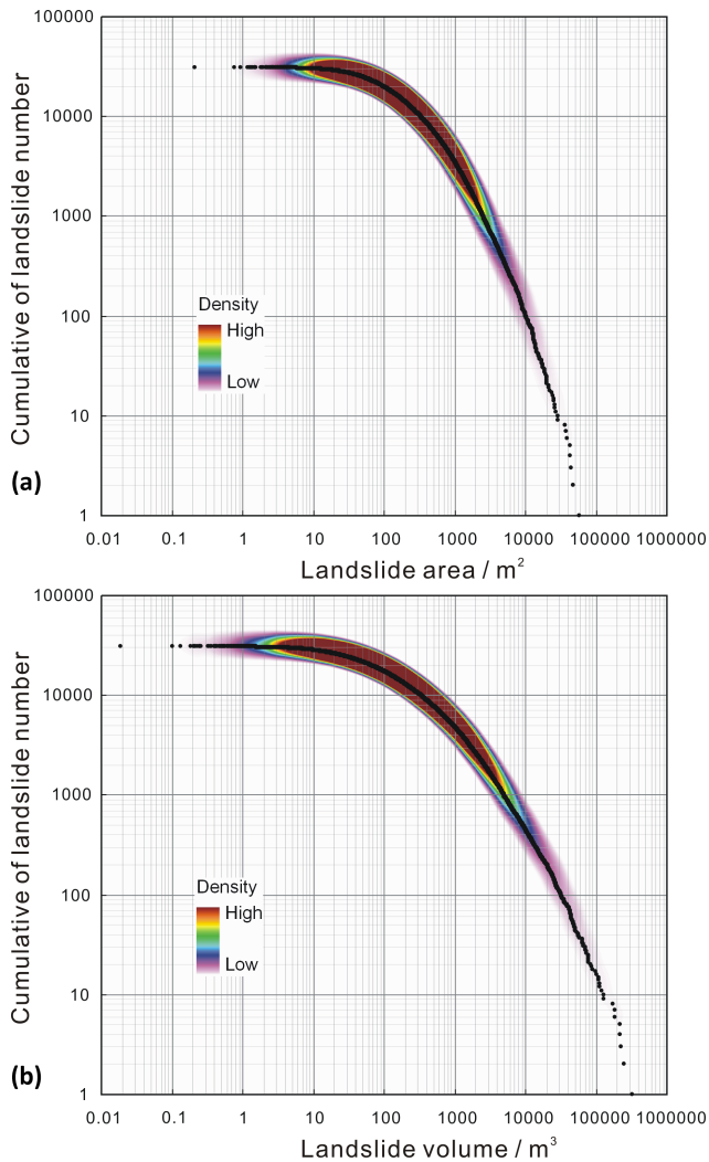
Figure 13. Correlations between cumulative landslide number and landslide scale: (a) landslide area and (b) landslide volume. Density means the density of points projected on the map, which represents the scale distribution of the landslide.
