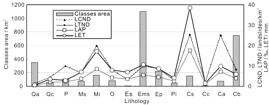
Figure 21. Relationships of landslide proxies with lithology.
