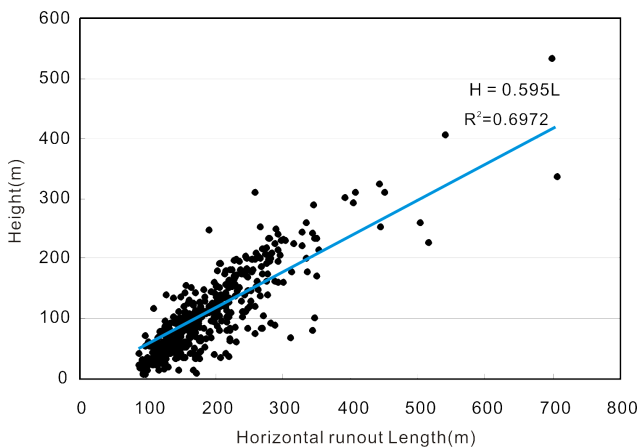
Figure 15. Relationship between landslide height and horizontal runout length. A total of 453 landslides of area larger than 10 000 m 2 triggered by the Haiti earthquake were used to carry out the statistics.
