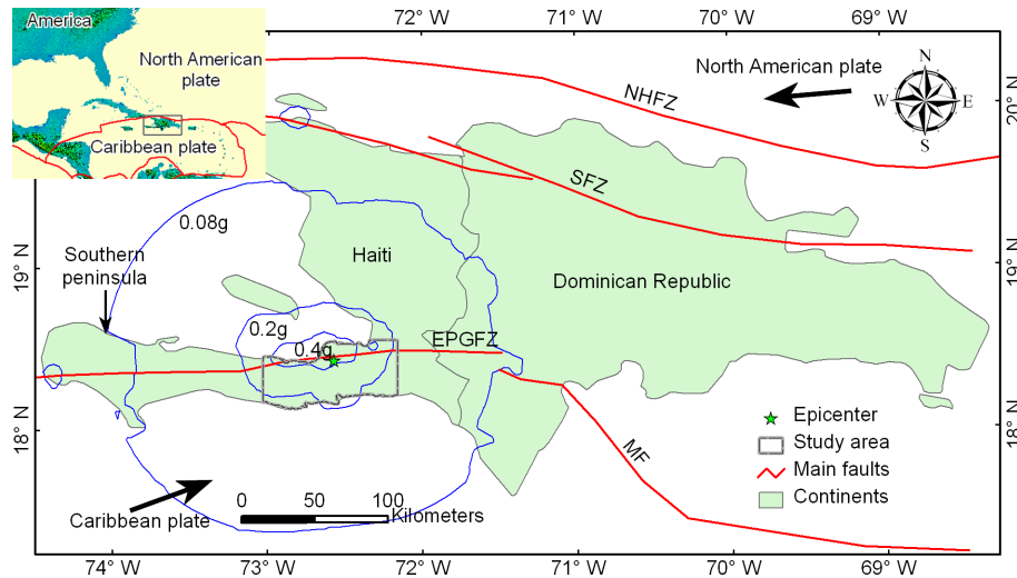
Figure 1. Location of study area, shown by the gray polygon. Thin blue lines indicate generalized PGA value contour lines. NHFZ: North Hispaniola fault zone; SFZ: Septentrional fault zone; EPGFZ: the Enriquillo–Plantain Garden fault zone; MF: Muertos fault.
