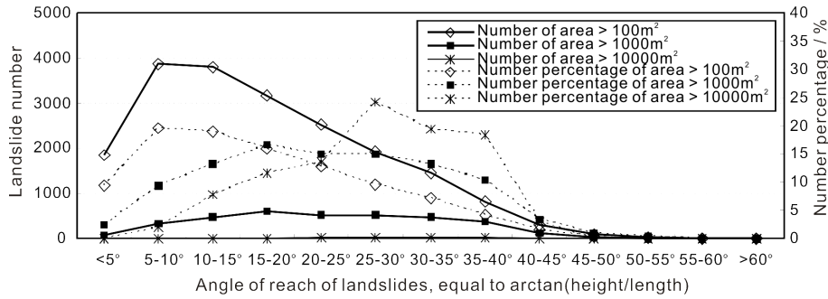
Figure 16. Landslide angle of reach [arctan(height/length)] distribution.
