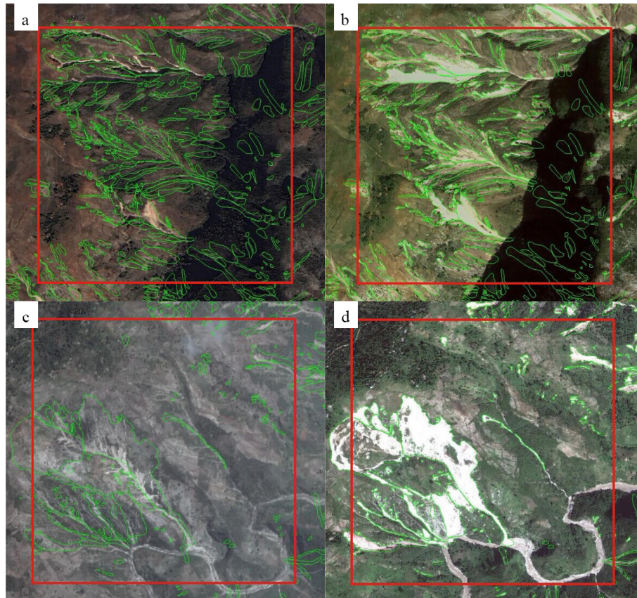
Figure 11. Examples of 1\text{ km} \times 1\text{ km} grids pre- and post-earthquake images. (a) taken on 4 February 2009, (b) taken on 21 January 2010, (c) taken on 2 June 2005, and (d) taken on 23 October 2010. The red square in (a) and (b) shows the grid of the largest landslide number density and landslide area percentage located in grid (a) in Fig. 10, and the red square in (c) and (d) shows the grid of the largest landslide erosion thickness located in grid (b) in Fig. 10.
