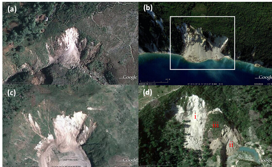
Figure 8. (a) and (b) are two rock falls occurred at (18^{\circ}28'07.75'' N, 72^{\circ}29'15.00'' W) and (18^{\circ}26'31.30'' N, 72^{\circ}49'44.20'' W), respectively. (a) was taken on 13 January 2010 (upward is northeast) and (b) was taken on 25 January 2010 (upward is south). (c) is located at 18^{\circ}28'51.78'' N, 72^{\circ}26'42.00'' W, and was taken on 13 January 2010 (upward is north). (d) shows several rock falls at 18^{\circ}19'38.90'' N, 72^{\circ}40'01.32'' W, and the images was taken on 25 January 2010 (upward is west).
