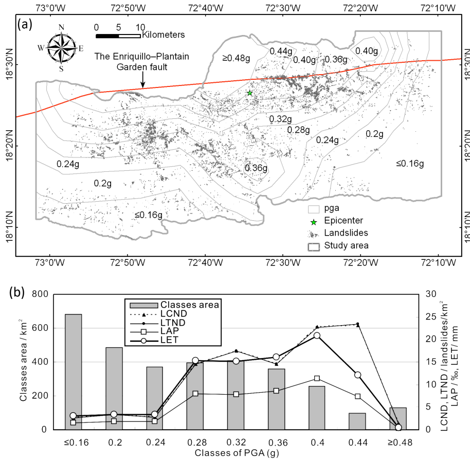
Figure 25. (a) Distribution of PGA values of the study area and (b) relationships of co-seismic landslides and PGA.
