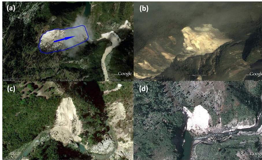
Figure 9. Several rock slides triggered by the Haiti earthquake. (a) shows a rock slide located at 18^{\circ}17'50.27'' N, 72^{\circ}38'38.01'' W; the image was taken on 25 January 2010 (upward is west). (b) is located at 18^{\circ}21'38.49'' N, 72^{\circ}42'14.65'' W; the image was taken on 14 January 2010 (upward is north). (c) is located at 18^{\circ}19'25.09'' N, 72^{\circ}39'07.99'' W; the image was taken on 25 January 2010 (upward is west). (d) is located at 18^{\circ}27'20.60'' N, 72^{\circ}24'19.85'' W, and the image was taken on 13 January 2010 (upward is west).
