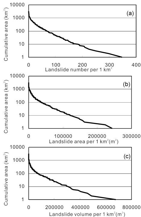
Figure 28. Curves of LND, LAP, and LET with the area distribution. (a) LND (centroid), (b) LAP, and (c) LET.
