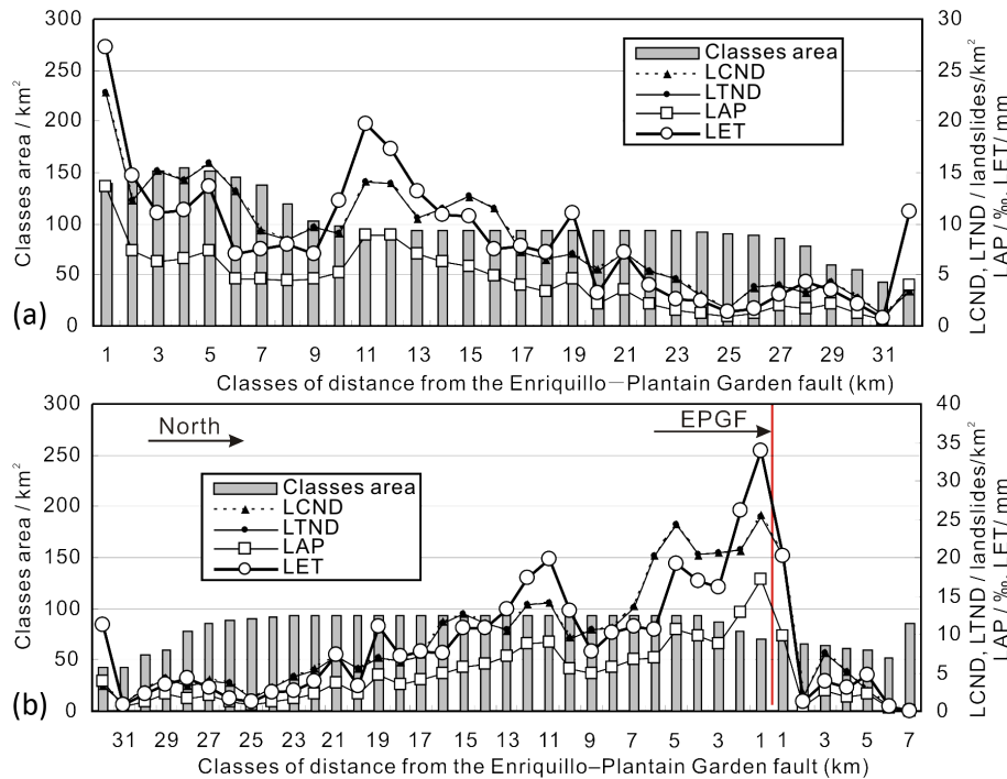
Figure 23. Relationships of co-seismic landslides and distance from the Enriquillo–Plantain Garden fault. (a) Without considering the differences on the two sides of the fault, (b) considering the differences on the two sides of the fault.
