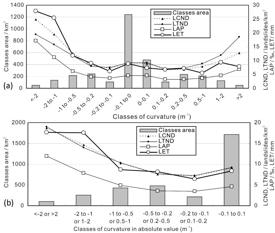
Figure 20. Relationships between co-seismic landslides and slope curvature. (a) Classes divided considering the sign of slope curvature, and (b) classes divided without considering the sign of slope curvature.
