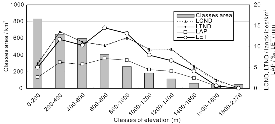
Figure 17. Relationship of co-seismic landslide abundances with elevations.
