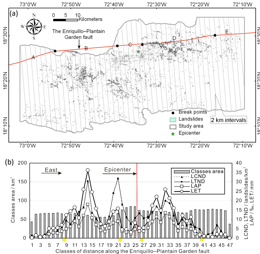
Figure 24. (a) Segments of the Enriquillo–Plantain Garden fault and 2 km bands for classifying distance along the fault. A: Miragoâne segment, B: Goave segment, C: Dufort segment, D: Momance segment, and E: Dumay segment. (b) Relation of co-seismic landslides and distance along the Enriquillo–Plantain Garden fault are also presented. In all, 47 classes with 2 km intervals were analyzed, and the epicenter is located between classes 25 and 26. The yellow points represent the boundaries of the five segments of the Enriquillo–Plantain Garden fault.
