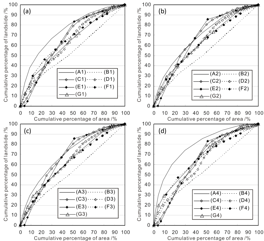
Figure 27. Cumulative landslide area curves to analyze the influence of the seven impact parameters on the landslide occurrences, separately shown by different landslide proxies. 1: landslide area, 2: landslide centroid point number, 3: landslide top point number, and 4: landslide accumulation material volume. The curves are: A: slope angle, B: slope curvature, C: distance from epicenter, D: distance from the Enriquillo–Plantain Garden fault, E: PGA, and F: distance from drainages.
