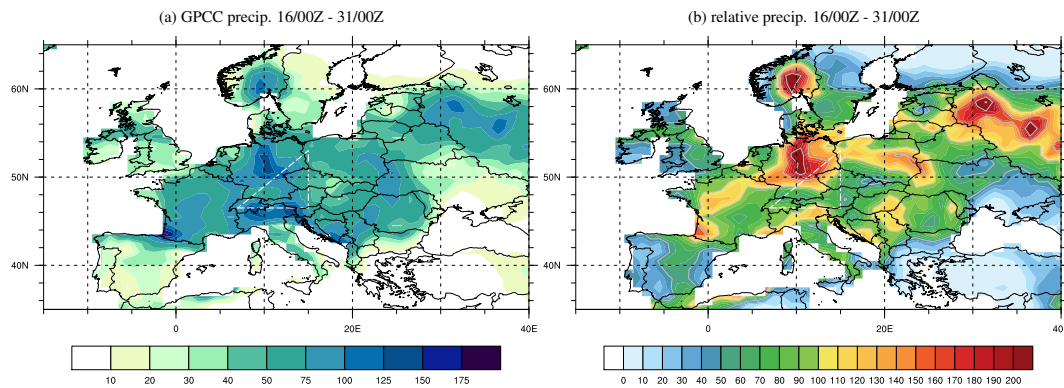
Figure 1. (a): observed precipitation over land (shaded in mm) from first guess GPCC data accumulated from 16 May 2013, 00:00 UTC to 31 May 2013, 00:00 UTC and (b): fraction of total climatological May precipitation that fell during this 15 day period (shaded every 10 %, blue < 50 %, green 50–100 %, yellow 100–150 %, red > 150 %).
