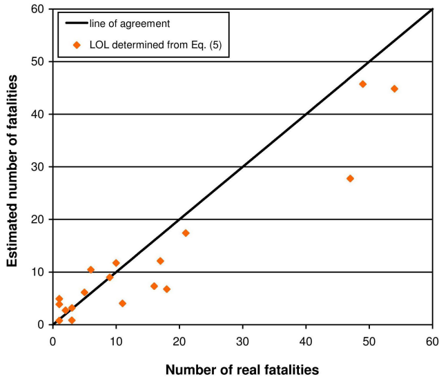
Figure 1. The degree of agreement between the real and calculated number of fatalities.
