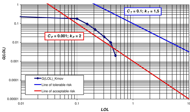
Figure 2. F–N curve for the Krnov locality.
