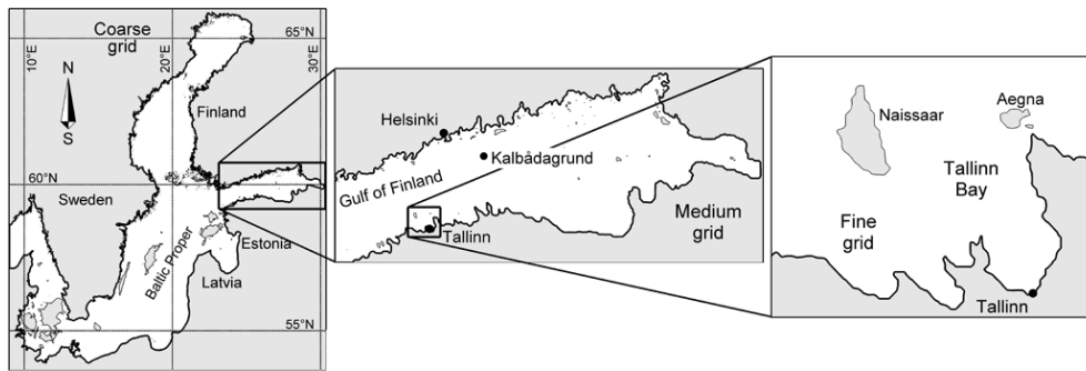
Fig. 1. Computational areas of the triple-nested wave model applied to the Tallinn Bay area.
