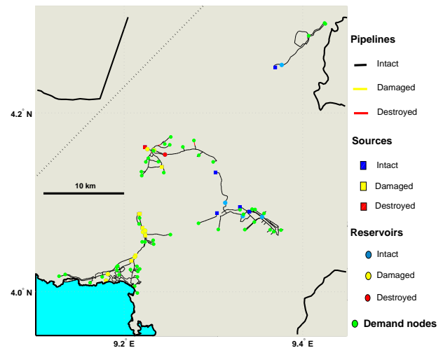
Fig. 11. Representation of the damage states of the water supply system components after the scenario presented in Fig. 5.
