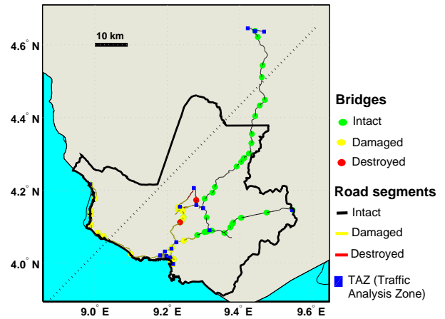
Fig. 10. Representation of the damage states of the road network components after the scenario presented in Fig. 5.
