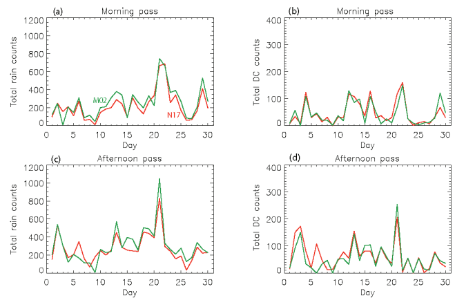
Fig. 4. Time series of October 2007 total (left) rain and (right) DC counts over the Mediterranean Basin for (top) morning and (bottom) afternoon NOAA-17/AMSU-B (N17, in red) and Metop-2/MHS (M02, in green) passes.
