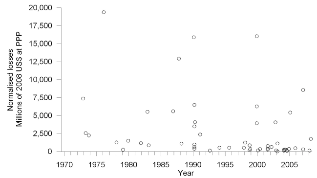
Fig. 2. Time-distribution of damaging windstorms included in the catalogue for Europe 1970–2008.
