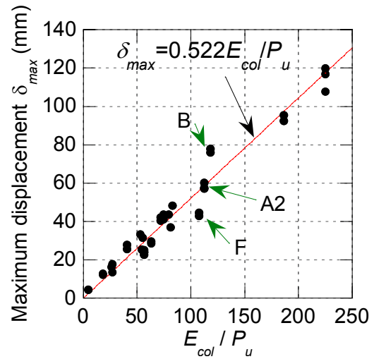
Fig. 14. Relationship between the ratio kinetic energy to ultimate bending capacity E_{col} / P_u and maximum displacement \delta_{max} .
