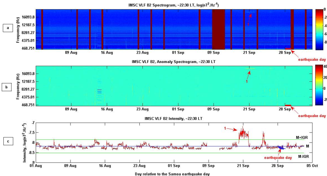
Fig. 3. Same as Fig. 2 but for IMSC VLF spectrogram of the B2 magnetic component.
