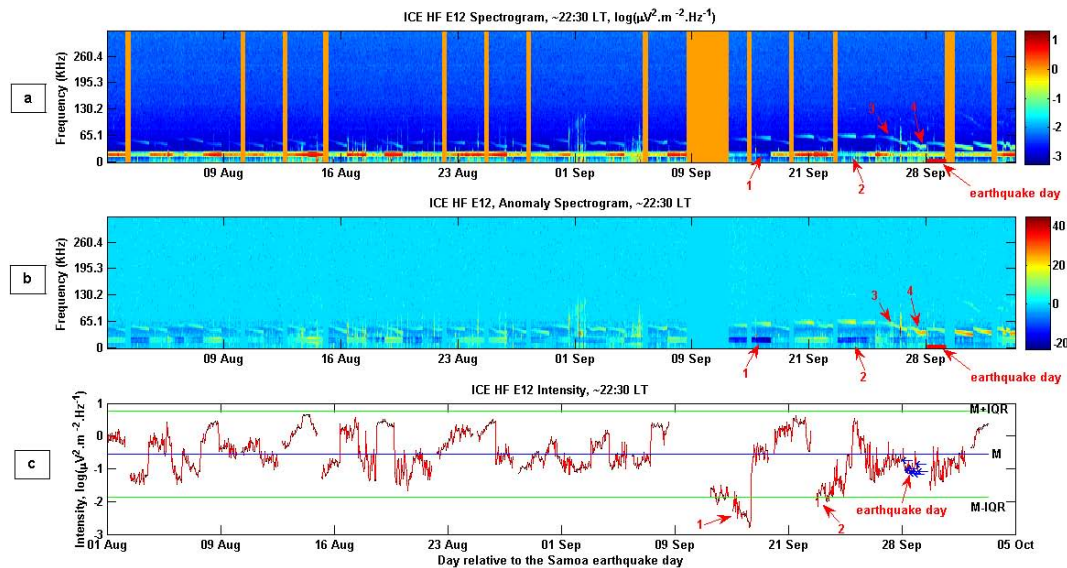
Fig. 4. Same as Fig. 2 but for ICE HF spectrogram of the E12 electric component.
