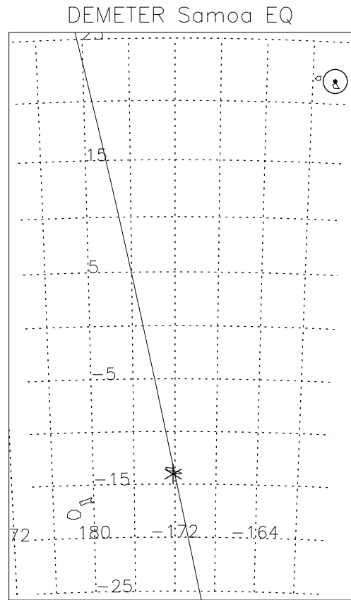
Fig. 1. Locations of the earthquake epicenter (*), of the VLF transmitter NPM (circle around a dot) and of one DEMETER orbit on 25 September 2009 (4 days before the event).
