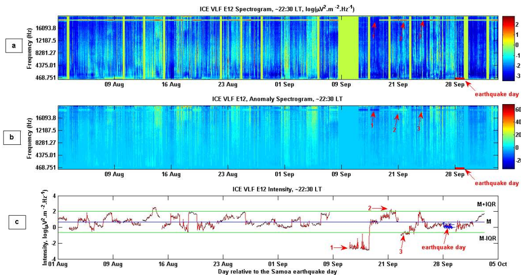
Fig. 2. Results of the DEMETER data analysis concerning the Samoa earthquake (29 September 2009) from 1 August to 5 October 2009 at \sim 22:30 LT. Due to the operation of satellite in safe mode a time gap is observed from 7 to 15 September 2009. The earthquake day is represented by a red tick below the X-axis. (a) ICE VLF spectrogram of the E12 electric component. The intensity of the spectrogram is color-coded according to the scale on the right. (b) Detected anomaly in the ICE VLF spectrogram of the E12 electric component. The anomaly is color-coded according to the scale on the right. (c) Intensity of ICE VLF spectrogram of the E12 electric component around the virtual NPM transmitter frequency (see text for explanation). For this panel the green horizontal lines indicate the higher and lower bounds ( M \pm IQR ). The blue horizontal line indicates the median value ( M ). In all panels, the X-axis represents days relative to the occurrence of the Samoa earthquake.
