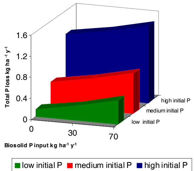
Fig. 11. P export under conditions of low connectivity but with a range of initial soil P conditions reflecting the history of P applications in a catchment
