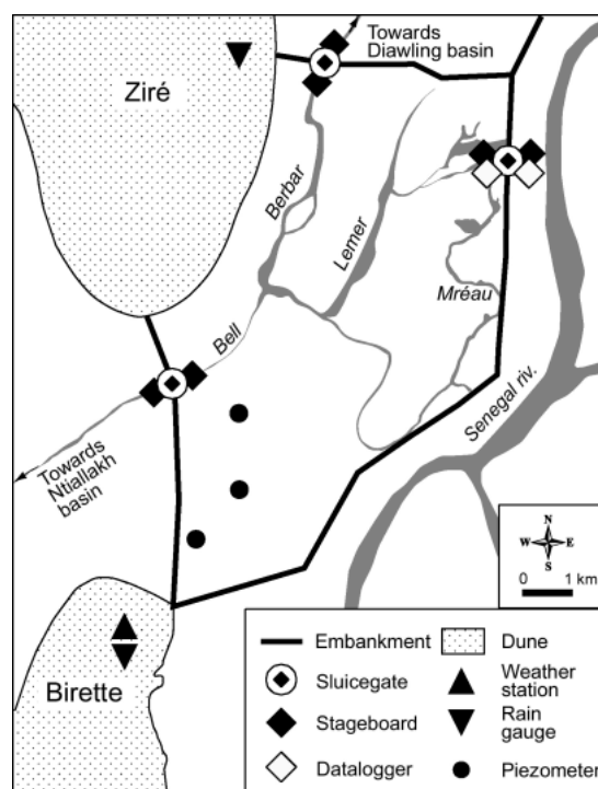
Fig. 5. Hydro-climatological framework for the Bell basin.
