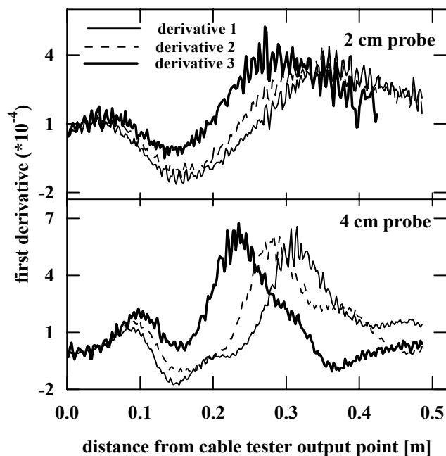
Fig. 2. First derivatives of the TDR waveforms shown in Fig. 1 for the 2 cm and 4 cm long probes.
