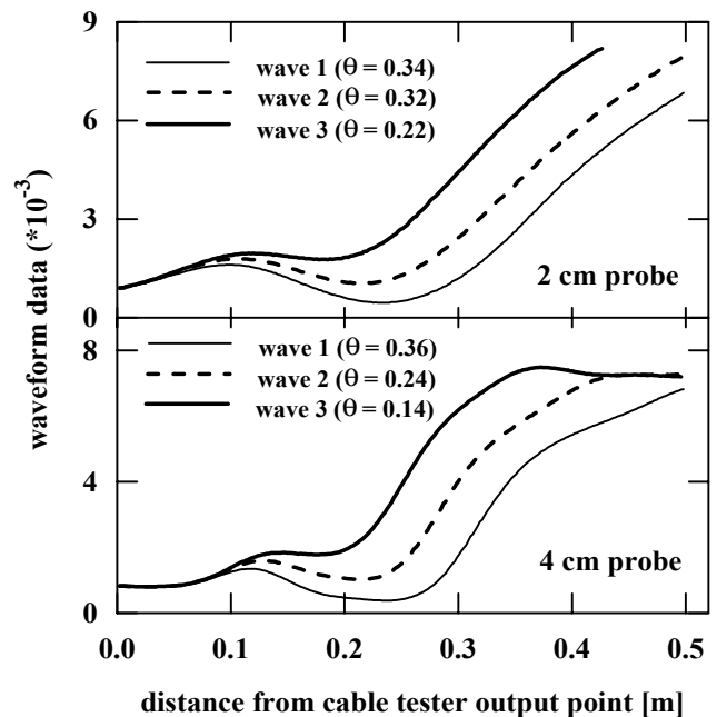
Fig. 1. TDR waveforms retrieved for three different soil-water contents in sand for a 2 cm and 4 cm long probe.
