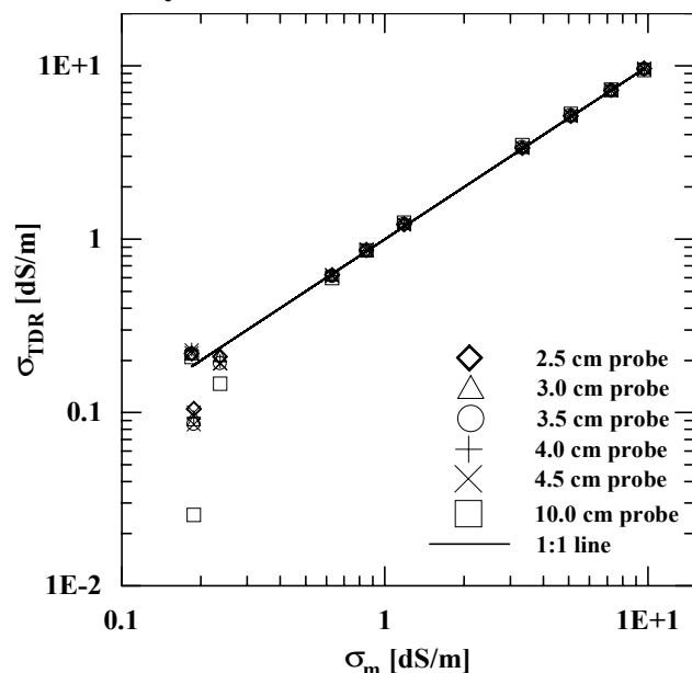
Fig. 4. Relationship between electrical conductivity of salt solutions measured by TDR probes \geq 2.5 cm in length s_{\text{TDR}} (dS m ^{-1} ) and electrical conductivity of the same salt solutions measured by a conductivity meter s_m (dS m ^{-1} ). The s_m - s_{\text{TDR}} relationship was linear in an arithmetic paper; the purpose of using log-log scale is to show the small values clearly.
