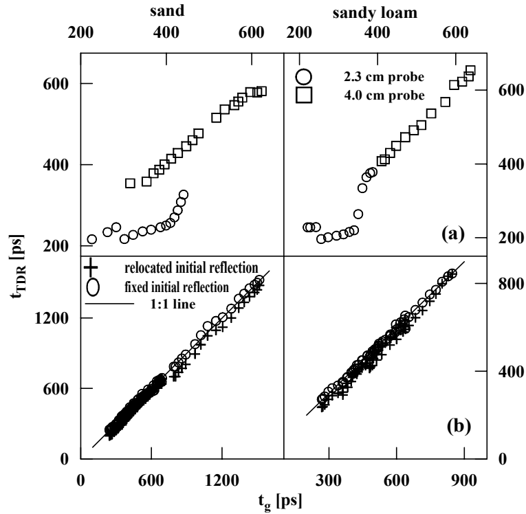
Fig. 3. Relationship between TDR-measured pulse travel time t_{TDR} and predicted pulse travel time t_g in sand and sandy loam soil for: (a) the fixed initial reflection of the TDR pulse on the waveforms of 2.3 cm and 4 cm long probes and (b) both fixed and relocated initial reflection of the TDR pulse on the waveforms of all probes = 2.5 cm in length.
