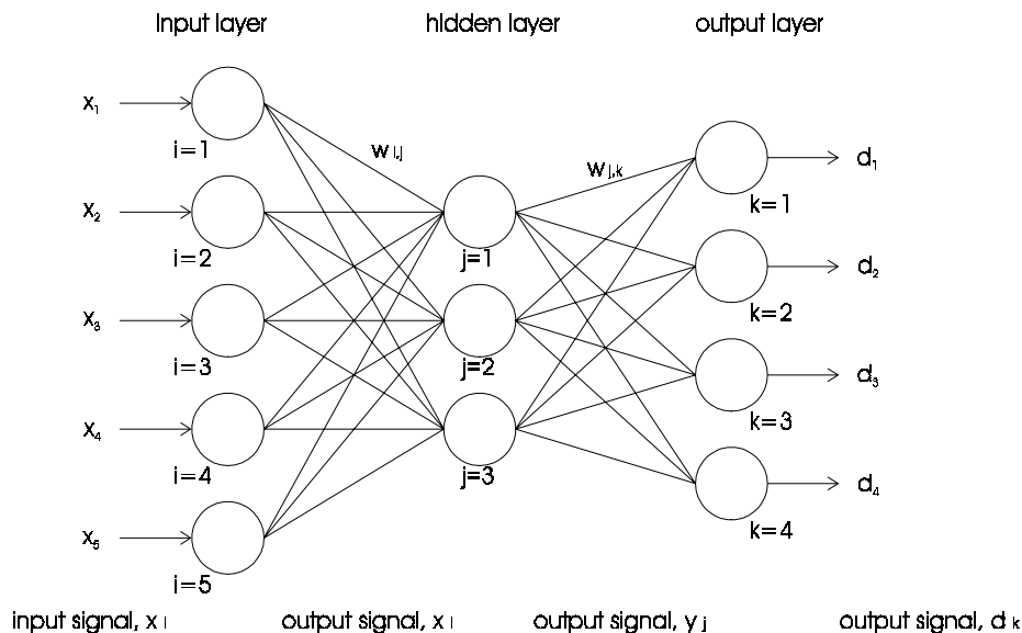
Fig. 1. A typical three-layer multi-layer perceptron (MLP) type neural network.
