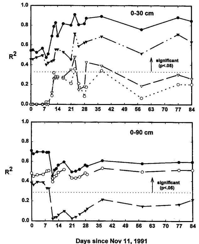
Fig. 3. Squared partial correlations for physiographic variables vs. soil moisture content during the measurement period. Physiographic variables shown are: topographic index ( \blacktriangledown -), soil storage index ( \circ -), and organic matter index ( \nabla -). Also shown are adjusted r^2 values for multiple regressions of physiographic variables on soil moisture ( \bullet -); only those variables that were significant in partial F tests ( p < .05 ) were included.
