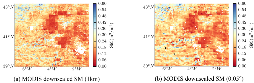
Figure 11. Spatial patterns of the downscaled soil moisture from MODIS at (a) 1 km and (b) 0.05° spatial resolutions.
