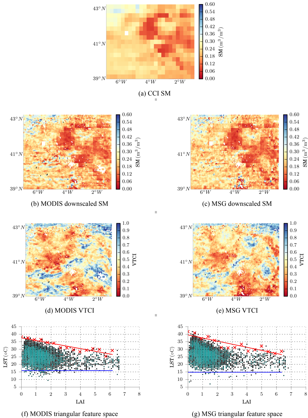
Figure 5. Spatial comparisons between coarse CCI soil moisture (a) and downscaled CCI soil moisture (b, c) based on MODIS and SEVIRI for 22 May 2010. The corresponding VTCI (d, e) and triangular/trapezoidal feature space (f, g) are also shown. The green points in the triangular feature space indicate the pixels with elevation 300 m higher or lower than the average REMEDHUS elevation.
