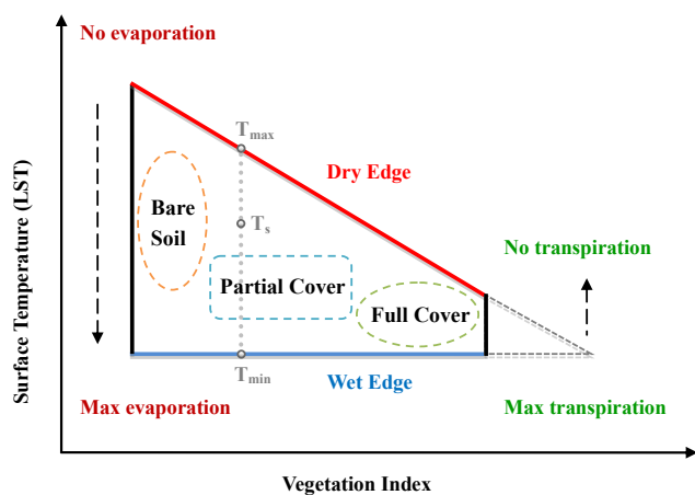
Figure 2. Conceptual diagram of the triangular/trapezoidal feature space that is constructed by land surface temperature and vegetation index.
