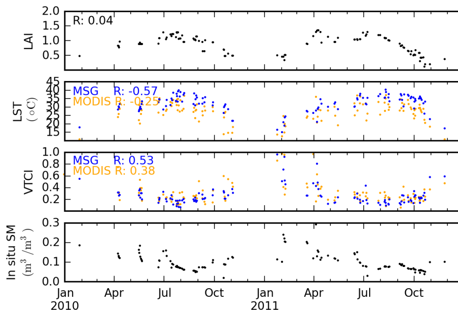
Figure 4. Time series of the station-averaged LAI, surface temperature, VTCI, and in situ soil moisture over REMEDHUS during the study period. The R values listed in the figure refer to the correlation coefficient with measured soil moisture.
