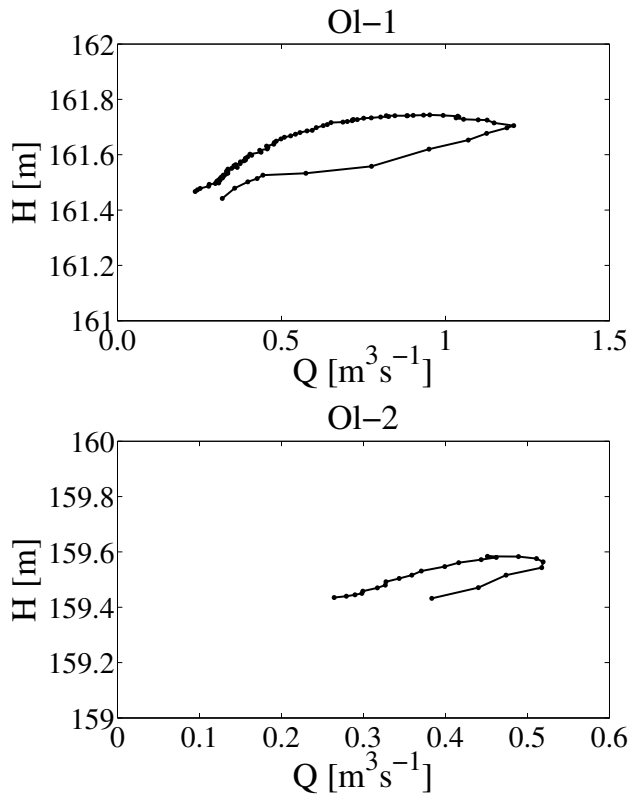
Figure 5. Rating curves of experimental flood waves in the Olszanka watercourse.
