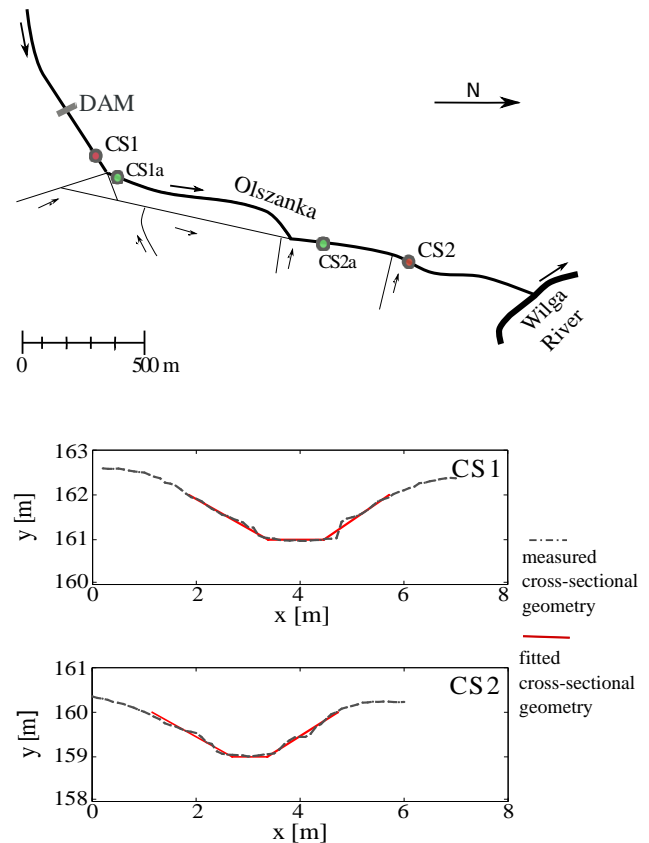
Figure 1. The site of the experiment in the Olszanka watercourse (upper panel), and the shape of measurement cross sections CS1 and CS2 (lower panel).
