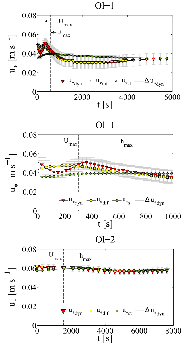
Figure 10. Comparison of friction velocity evaluated by formulae for dynamic u_{*dyn} , diffusive wave u_{*dif} and steady uniform flow u_{*st} with uncertainty bounds \Delta u_{*dyn} for experimental flood waves in the Olszanka watercourse. Middle panel shows an enlargement of the rising limb of the wave for Ol-1.
