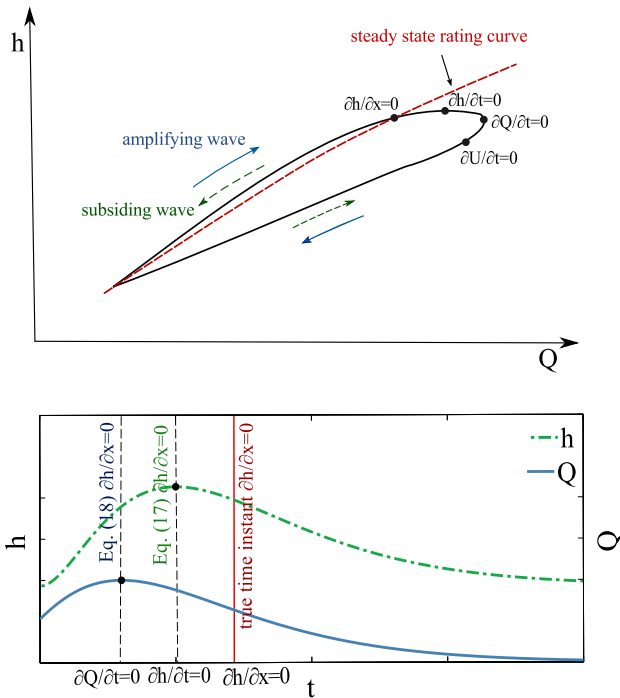
Figure 6. Comparison between rating curve for flood wave and steady flow with characteristic points, based on Henderson (1963) (upper panel), and impact of kinematic wave approximation (Eqs. 17, 18) on the assessment of time instant at which \frac{\partial h}{\partial x} = 0 (lower panel).
