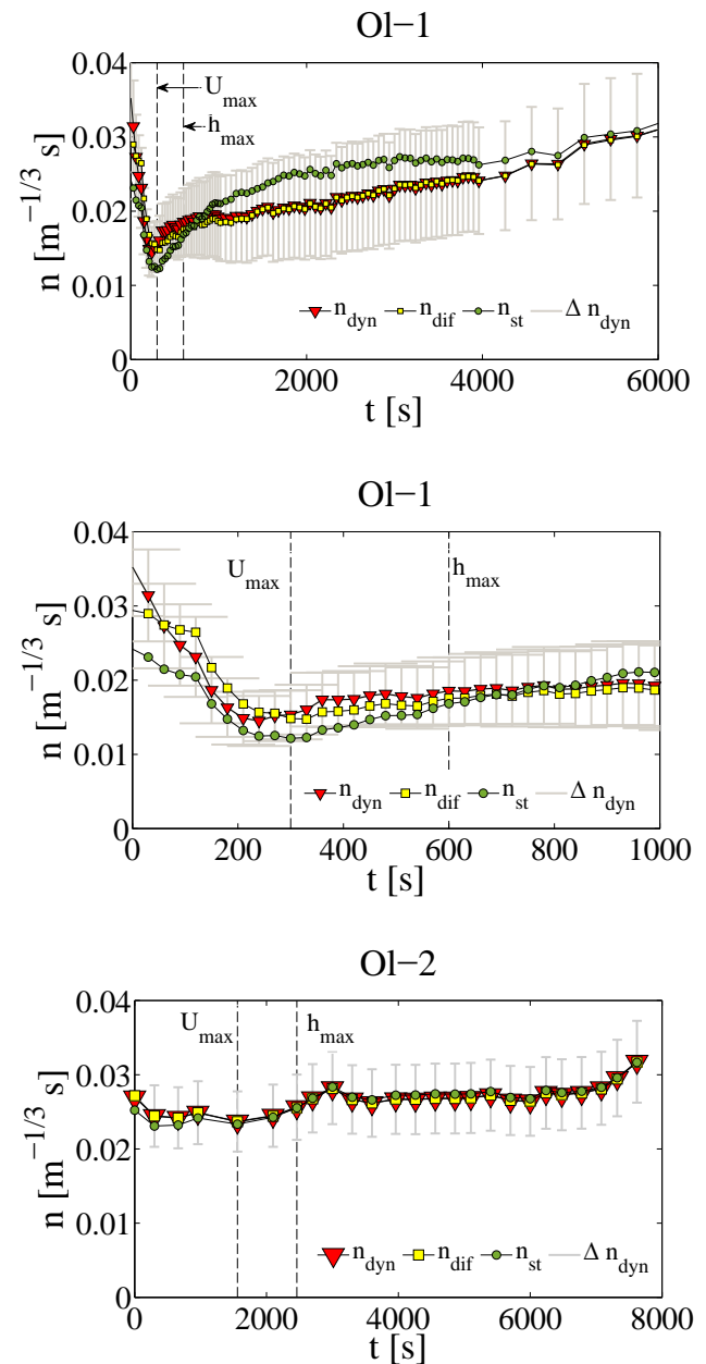
Figure 11. Comparison of n evaluated by formulae for dynamic n_{\text{dyn}} , diffusive wave n_{\text{dif}} and steady uniform flow n_{\text{st}} with uncertainty bounds \Delta n_{\text{dyn}} for experimental flood waves in the Olszanka watercourse. Middle panel shows an enlargement of the rising limb of the wave for Ol-1.
