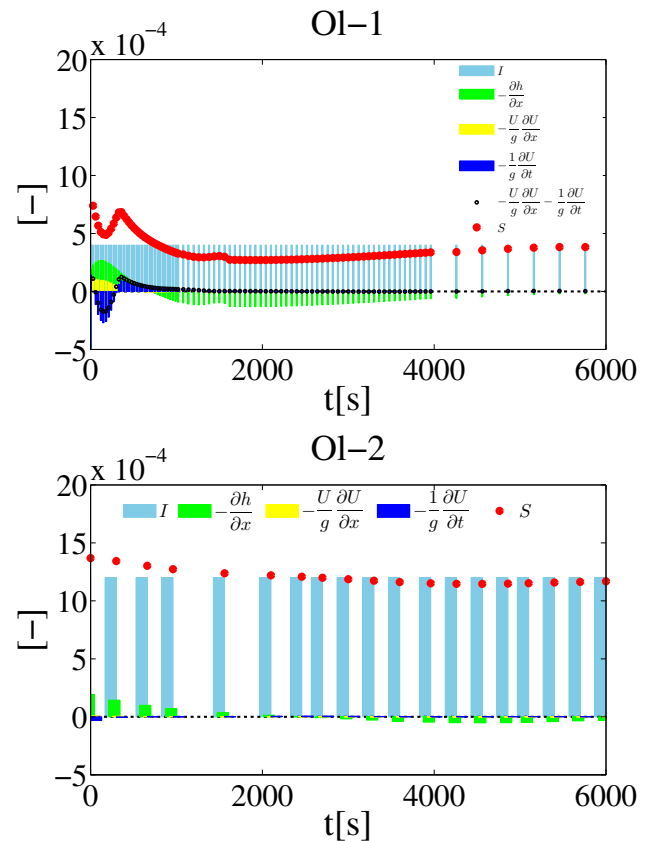
Figure 8. Comparison of terms of the momentum balance equation for experimental flood waves in the Olszanka watercourse.
