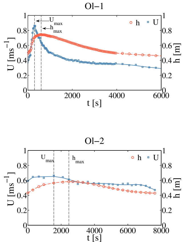
Figure 4. Temporal variability of flow depth h and mean velocity U for experimental flood waves in the Olszanka watercourse.
