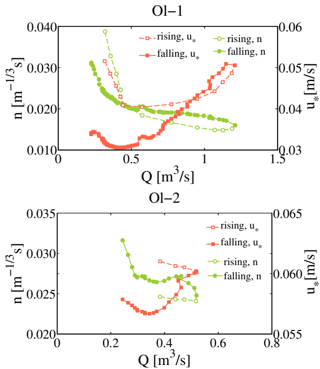
Figure 12. Comparison of the relation of n vs. flow rate Q and friction velocity u_* vs. Q along rising and falling limbs of waves for experimental flood waves in the Olszanka watercourse.
