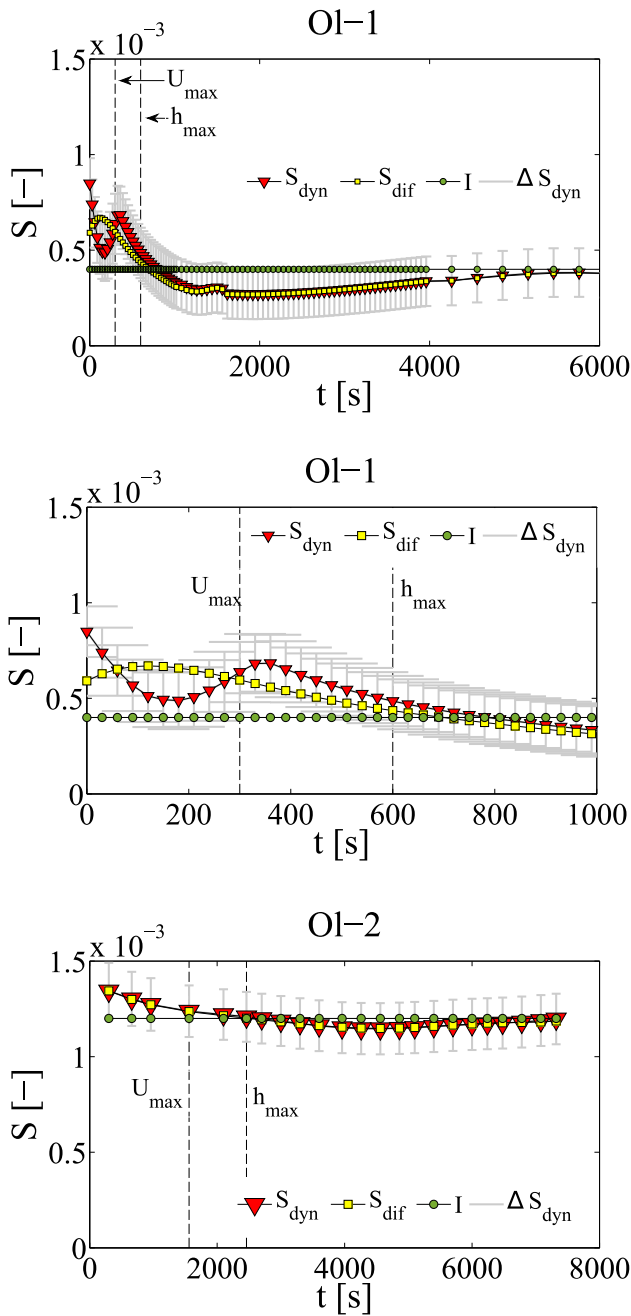
Figure 9. Comparison of friction slope evaluated by formulae for dynamic S_{dyn} , diffusive wave S_{dif} and steady flow I with uncertainty bounds \Delta S_{dyn} for experimental flood waves in the Olszanka watercourse. Middle panel shows an enlargement of the rising limb of the wave for Ol-1.
