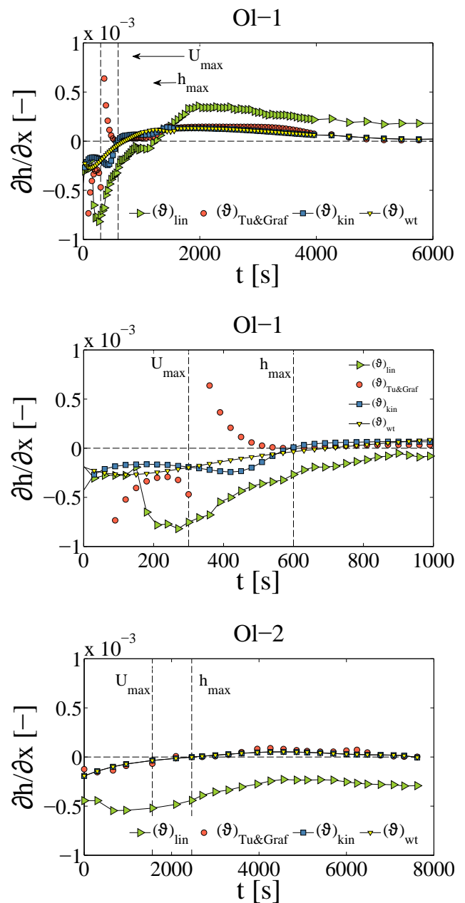
Figure 7. Temporal variability of gradient of flow depth \vartheta = \frac{\partial h}{\partial x} for experimental flood waves in the Olszanka watercourse. Middle panel shows an enlargement of the rising limb of the wave for Ol-1.
