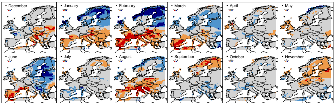
Figure 3. Monthly frequency trends in wet STs significant at the 70 % (light colours) and 95 % (dark colours); increasing trends in blue, decreasing trends in red.
