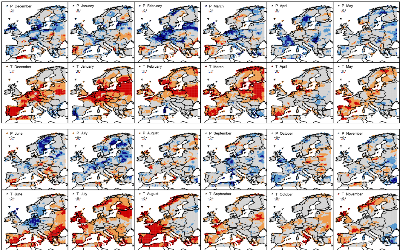
Figure 4. Monthly trends within the groups of wet STs for precipitation (rows 1 and 3) and temperature (rows 2 and 4) significant at the 70 % (light colours) and 95 % (dark colours). Precipitation: increasing trends in blue, decreasing trends in red. Temperature: increasing trends in red, decreasing trends in blue.
