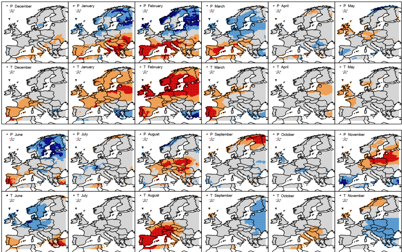
Figure 1. Synoptic-circulation-induced trends for precipitation (rows 1 and 3) and temperature (rows 2 and 4) significant at the 70 % (light colours) and 95 % (dark colours). Precipitation: increasing trends in blue, decreasing trends in red. Temperature: increasing trends in red, decreasing trends in blue.
