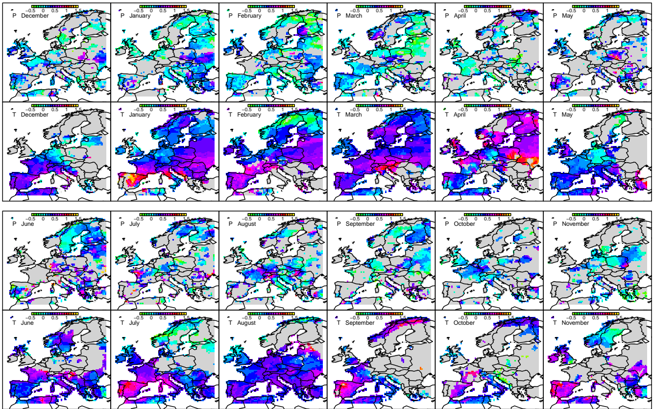
Figure 7. Monthly trend ratios for trends within the groups of dry STs for precipitation (rows 1 and 3) and temperature (rows 2 and 4).
