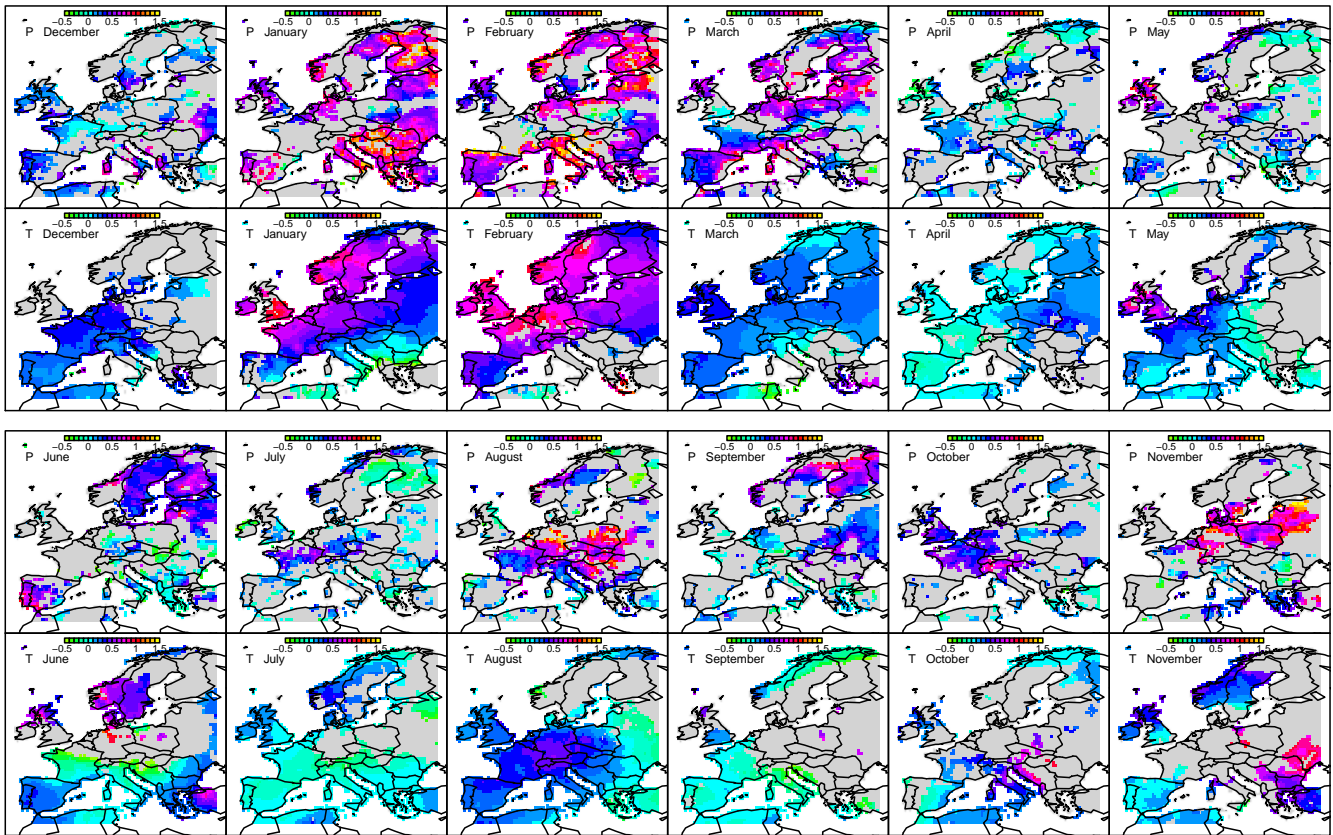
Figure 2. Monthly trend ratios for synoptic-circulation-induced trends in precipitation (rows 1 and 3) and temperature (rows 2 and 4).
