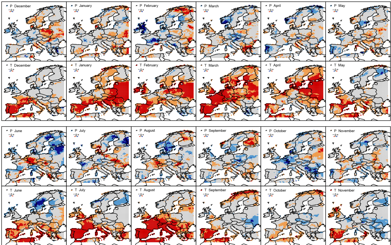
Figure 5. Monthly trends within the groups of dry STs for precipitation (rows 1 and 3) and temperature (rows 2 and 4) significant at the 70 % (light colours) and 95 % (dark colours). Precipitation: increasing trends in blue, decreasing trends in red. Temperature: increasing trends in red, decreasing trends in blue.
