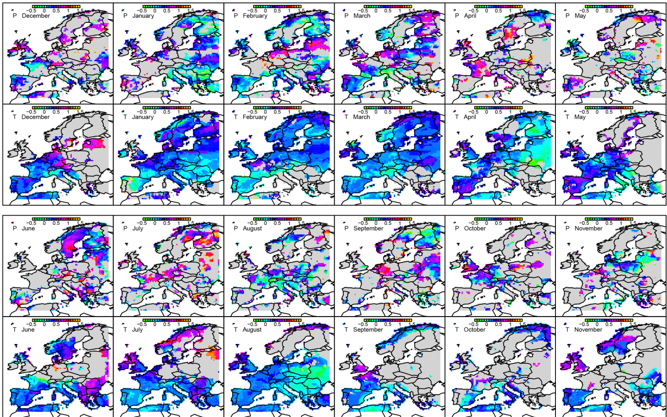
Figure 6. Monthly trend ratios for trends within the groups of wet STs for precipitation (rows 1 and 3) and temperature (rows 2 and 4).
