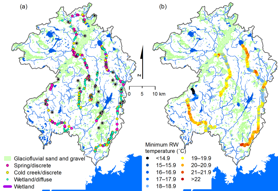
Figure 4. (a) Thermal anomalies identified in the AIR surveys in 2010 and 2011. (b) The longitudinal profiles of T_{\min r} of the rivers Vantaa, Keravanjoki and Lepsämäenjoki in 2011. (Basemap Database © National Land Survey of Finland 2010; Quaternary Deposit Database © Geological Survey of Finland 2008; Watershed Database © SYKE 2010.)
