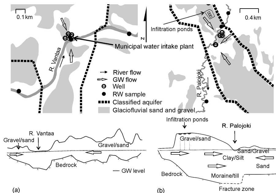
Figure 3. Schematic diagrams of the field study sites: (a) Hyvinkäänkylä field study site (bedrock elevation data from Breilin et al., 2004), and (b) River Palojoiki field study site (modified from Kortelainen and Karhu, 2006). (Basemap Database ® National Land Survey of Finland 2010; Quaternary Deposit Database ® Geological Survey of Finland 2008; Groundwater Database ® SYKE 2010; Watershed Database ® SYKE 2010.)
