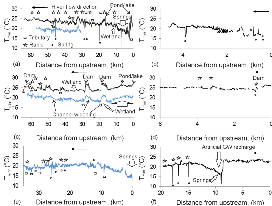
Figure 5. Longitudinal profiles of T_{\min r} of the rivers Vantaa (a), Herajoki (b), Keravanjoki (c), Tuusulanjoki (d), Lepsämäenjoki (e) and Palojoki (f) in 2010 (black line) and 2011 (blue line). Notable tributary confluences, GW–SW exchange, dams, rapids and channel morphology changes are marked in profiles.
