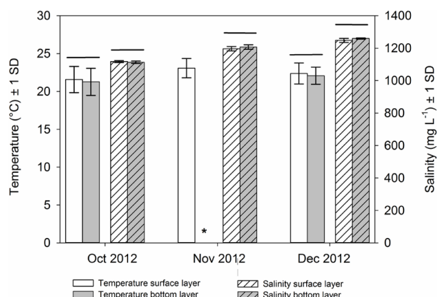
Figure 2. Temperature (°C) and salinity (ppm) in the surface and bottom layers measured at seven sites over three months in Lake Yangebup during a previous study in 2012. “***” indicates missing data; horizontal line indicates that no significant difference between layers were detected ( t -test) (from Song et al., 2015).
