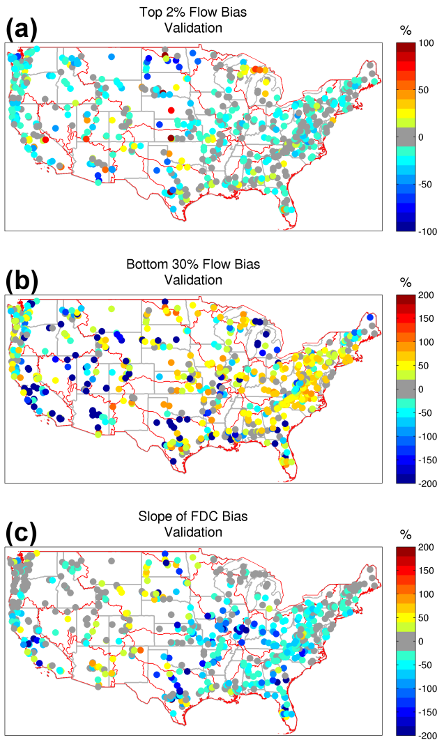
Figure 6. (a) Spatial distribution of the high flow bias, (b) low flow bias, and (c) flow duration curve bias for the validation period.
