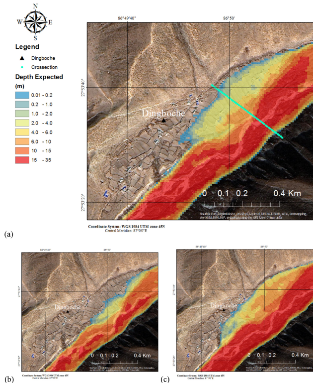
Figure 6. Inundation at Dingboche under current lake conditions: (a) expected inundation and the location of the cross section where the different scenarios are compared, (b) lower bound and (c) upper bound of the possible inundation.
