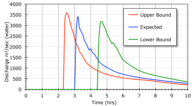
Figure 7. Upper bound, expected and lower bound GLOF hydrograph under current conditions at Phakding.
