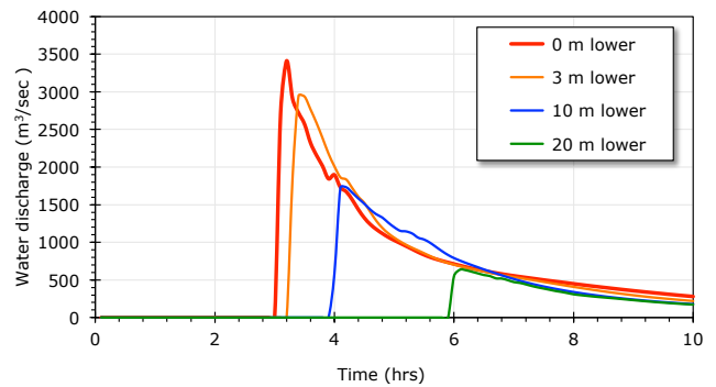
Figure 11. GLOF hydrographs at Phakding under current conditions for 0, 3, 10 and 20 m lake lowering scenarios.
