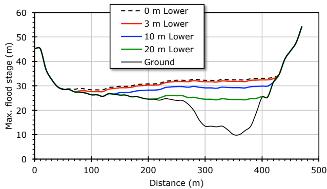
Figure 9. GLOF flood stage at Dingboche under current lake conditions for 0 m (expected), 3, 10 and 20 m lake lowering scenarios.
