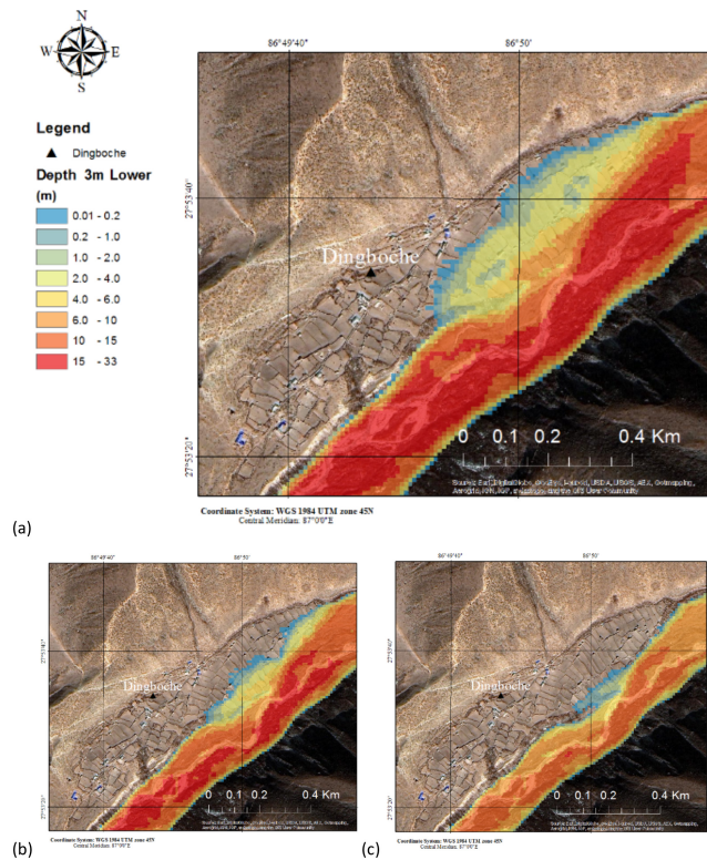
Figure 10. Inundation depth at Dingboche under current lake conditions: (a) 3 m lake lowering, (b) 10 m lake lowering and (c) 20 m lake lowering.
