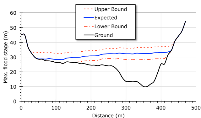
Figure 5. Upper bound, expected and lower bound GLOF flood stage at Dingboche (cross section shown in Fig. 4) under current conditions.
