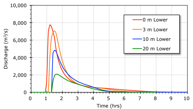
Figure 8. GLOF hydrographs at Dingboche under current lake conditions for 0, 3, 10 and 20 m lake lowering scenarios.
