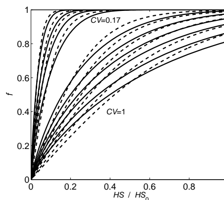
Figure 9. Snow-cover depletion curves derived assuming normally distributed snow depth and homogeneous melt via Eq. (4) as function of mean HS normalized with the peak of winter mean snow depth \text{HS}_0 (indicated by the subscript 0) (solid lines). Dashed lines represent parameterized fractional SCA f via Eq. (7). Coefficient of variations CV vary between 0.06 (upper left) and 1 (lowest one).
