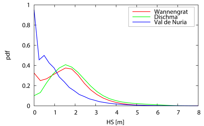
Figure 2. Probability density functions (pdf) of measured snow depths are shown for the three areas.
