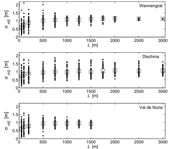
Figure 5. Standard deviation of snow depth \sigma_{HS} as function of domain size L for all three areas. The squares represent mean \sigma_{HS} .
