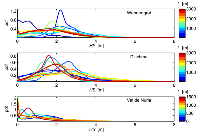
Figure 3. One example probability density function (pdf) of measured snow depths HS for each domain size L (in color) in each area.
