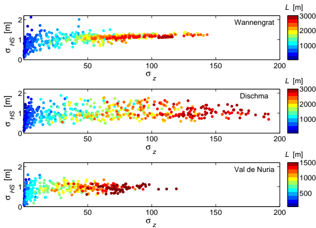
Figure 6. Standard deviation of snow depth \sigma_{HS} as a function of detrended valley-to-peak elevation difference \sigma (indicated by \sigma_z ) of the underlying topographic features. Colors indicate corresponding domain size L .
