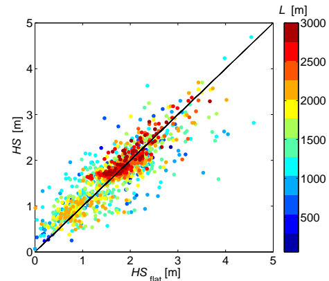
Figure 7. Measured mean snow depth HS as function of mean measured flat field HS_{flat} for all three areas. Colors indicate corresponding domain size L .
