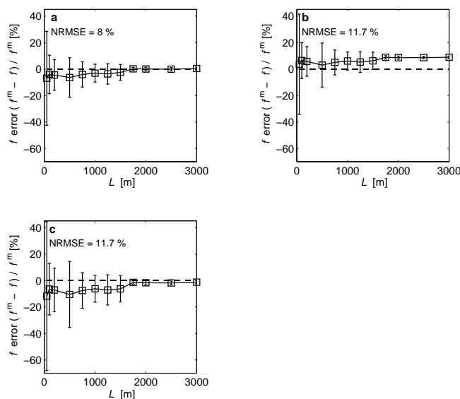
Figure 10. Error in fractional SCA f between measured f^m and parameterized f (Eq. 7) as function of the domain size L for all three areas. (a) Parameterized using \sigma_{\text{HS}} from Eq. (2), (b) parameterized using \sigma_{\text{HS}} from Egli and Jonas (2009) and (c) parameterized using \sigma_{\text{HS}} from Pomeroy et al. (2004). Mean values are indicated by squares. Error bars show the standard deviation of the error per L . NRMSEs are given for each parameterization.
