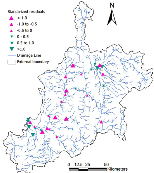
Figure 7. Model residuals for 31 monitoring stations used to calibrate the final Ishikari SPARROW model.
