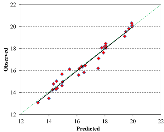
Figure 6. Observed and predicted SS flux ( \text{kg yr}^{-1} ) at 31 monitoring sites included in the Ishikari SPARROW model (Natural logarithm transformation applied to observed and predicted values; the black line is the trend line, the green dashed line is a 1 : 1 line).
