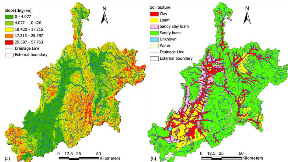
Figure 5. Schematic showing the slope (a) and soil texture (b) in the Ishikari River basin.
