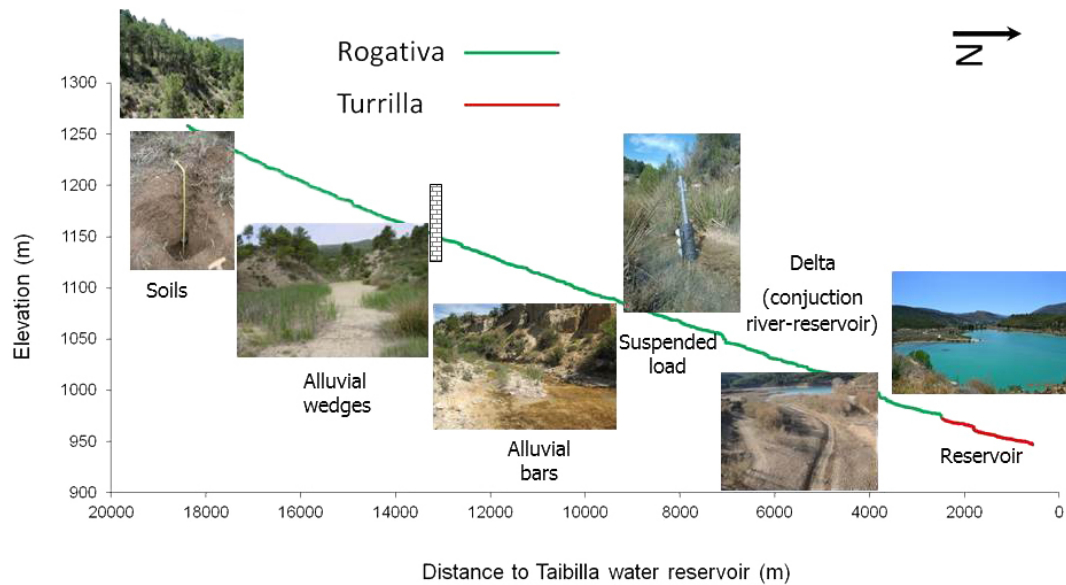
Figure 2. Sketch representing the morphological positions selected for sampling of soil and sediments. Soils were sampled all around the catchment in all the different land use classes, alluvial wedges behind check dams predominantly in the upper and middle parts of the catchment, while alluvial bars and suspended solids were sampled in the middle and downstream areas. Delta and reservoir represent sampling areas downstream.
