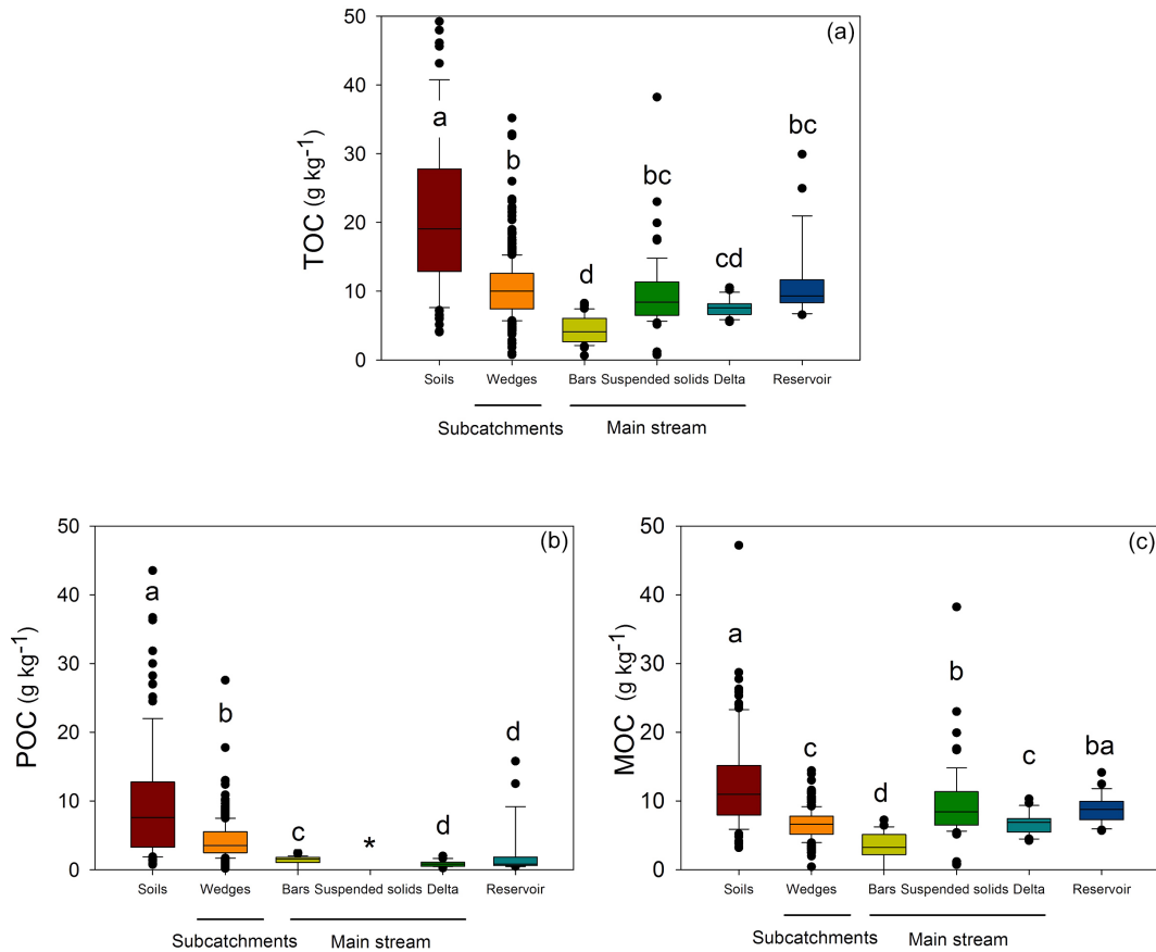
Figure 4. Median, percentiles (10th, 25th, 75th and 90th) and error of the total organic carbon concentration (TOC) (A), particulate organic carbon (POC) (B), and mineral associated organic carbon (MOC) (C) of soils and sediments within the Turrilla catchment. Different letters (a–e) indicate significant differences according to the Kruskal–Wallis test ( p < 0.05 ). * – the suspended solids measured contained only the MOC fraction.
