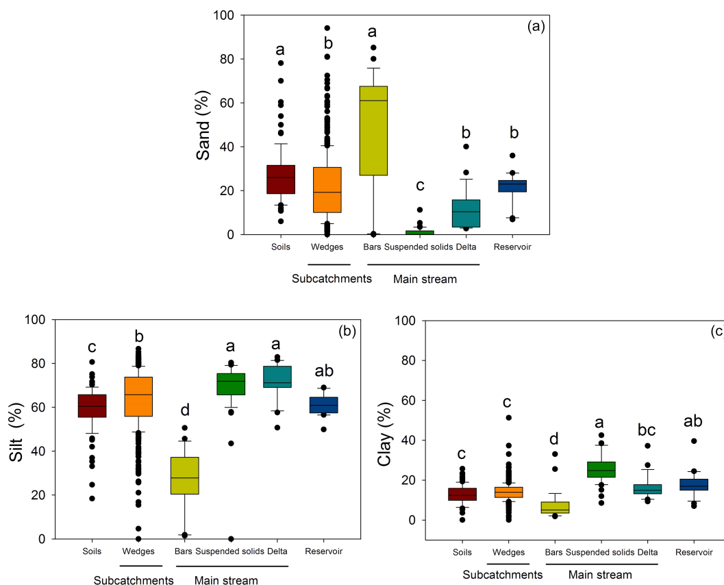
Figure 3. Median, percentiles (10th, 25th, 75th and 90th) and error of the main textural classes (A, sand; B, silt; C, clay) of the different types of sedimentary deposits within the Turrilla catchment. Different letters mean significant differences according to the Kruskal–Wallis test ( p < 0.05 ).
