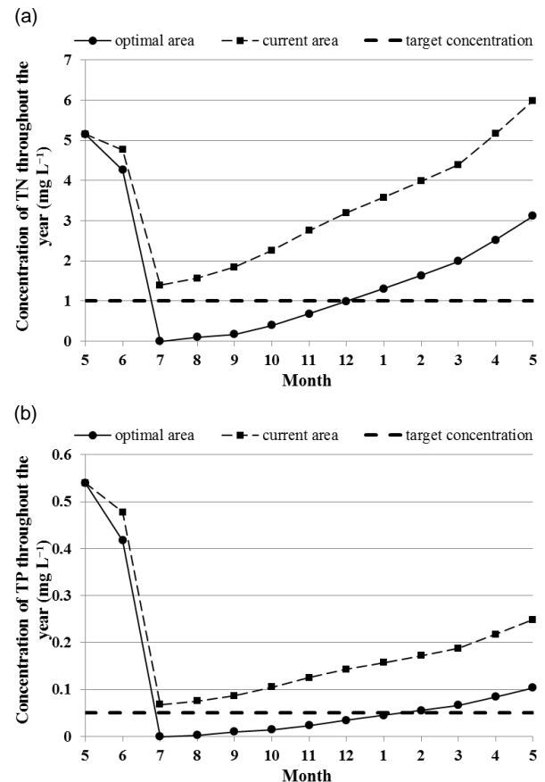
Figure 1. Lake water quality throughout the year under the optimal and current reed areas.
