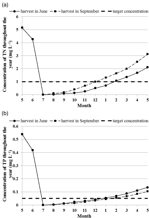
Figure 2. Lake water quality throughout the year under different harvest schemes.
