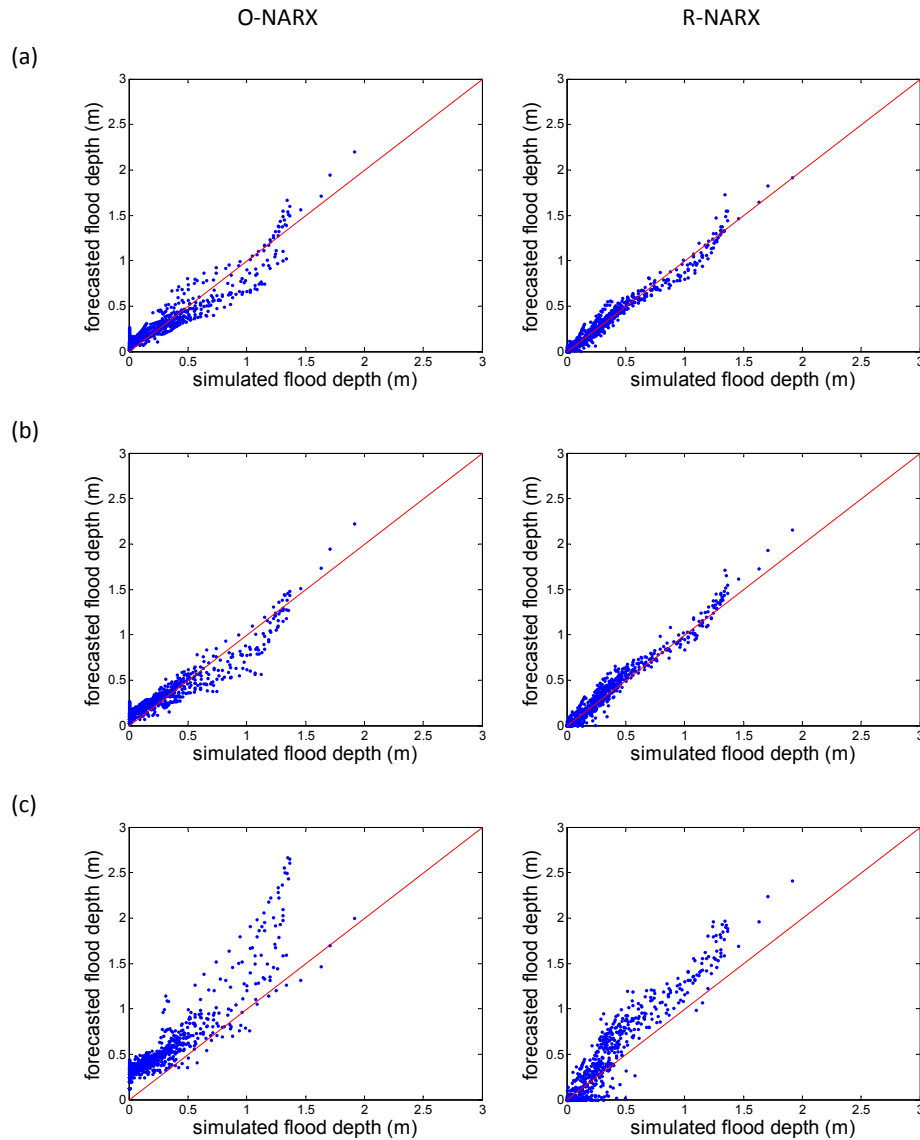
Fig. 6. Comparison of simulated and (a) one-hour-ahead, (b) three-hour-ahead, (c) six-hour-ahead forecasted inundation depths of the O-NARX and R-NARX models during the testing phase at S2.
