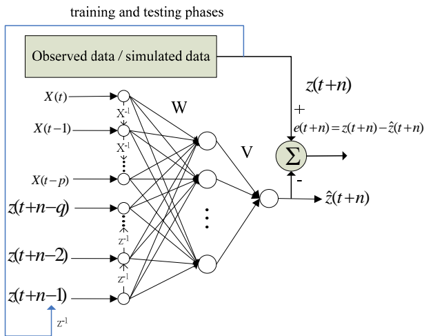
Fig. 1. Architecture of the T-NARX network during training and testing phases in the time delay mode.
