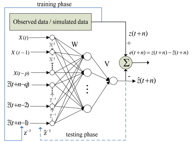
Fig. 2. Architecture of the O-NARX network during training and testing phases in the online time delay mode.
