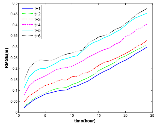
(a) O-NARX
