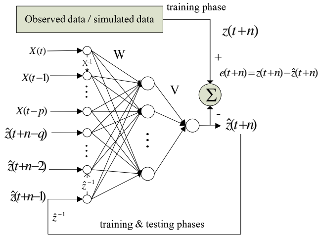
Fig. 3. Architecture of the R-NARX network during training and testing phases in the recurrent mode.
