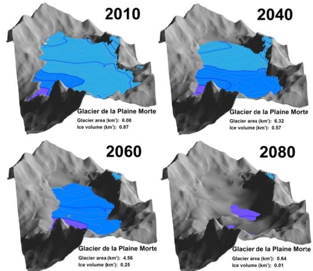
Fig. 10. Modeled future retreat of the Plaine Morte in 2010, 2040, 2060, and 2080. Colors indicate surface elevation bands of the glacier. The glacier area and volume for each time slice are indicated in the panels.
