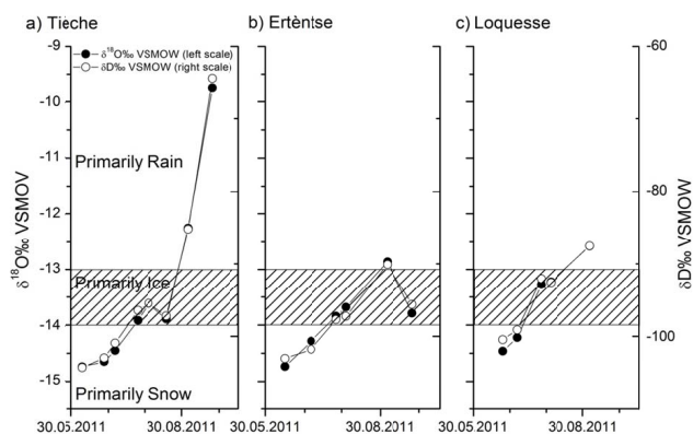
Fig. 8. Temporal development of isotopic composition at selected karst springs south of the Plaine Morte. Typical isotopic signatures found in ice samples are illustrated with striped area. Locations are shown in Fig. 1.
