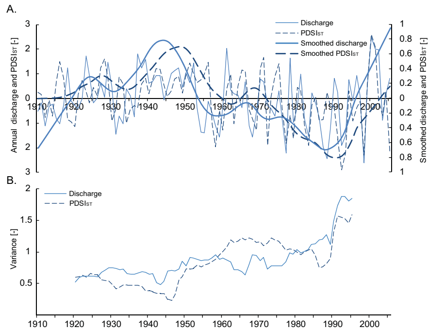
Fig. 2. Comparison of standardised basin averaged PDSI ( PDSI_{ST} ) and discharge for Stung Treng over the period 1910–2005: (A) annual values and LOESS smoothed values; and (B) moving variances with a 21 yr window.
