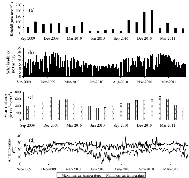
Fig. 3. The (a) monthly rainfall, (b) daily solar radiant density, (c) monthly solar radiant density, and (d) daily maximum and minimum air temperatures at the Mfabeni Mire.
