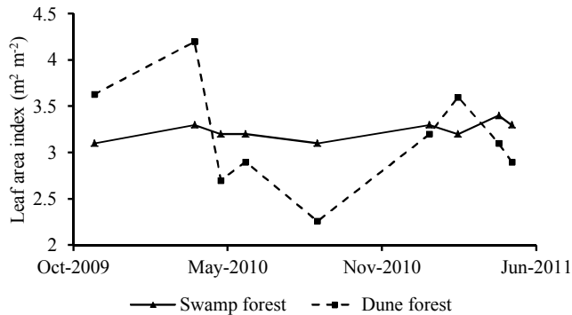
Fig. 2. Leaf area index measured at the swamp forest (above the ferns) and dune forest sites.
