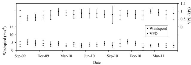
Fig. 4. Monthly average vapour pressure deficit and wind speed with standard deviation error bars measured at the Mfabeni Mire during daylight hours.
