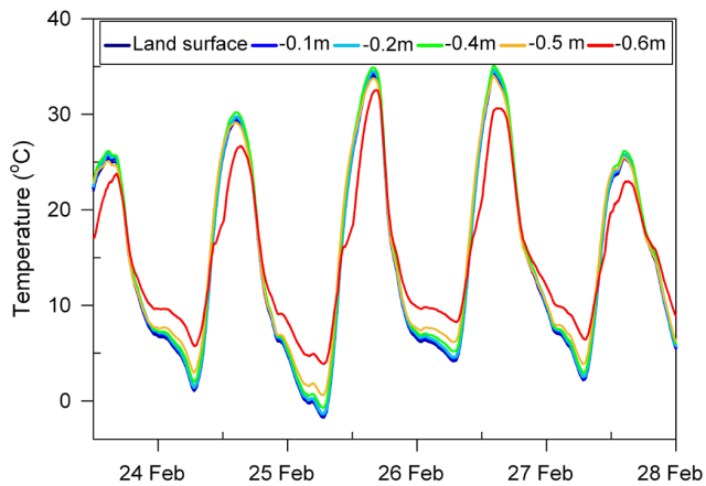
Fig. 7. Daily fluctuations in the temperature profile inside desiccation cracks at the study site. Each line represents a different temperature sensor and its depth, relative to the land surface. Note the unstable conditions (cold air above warm air) that develop in the cracks every night.
