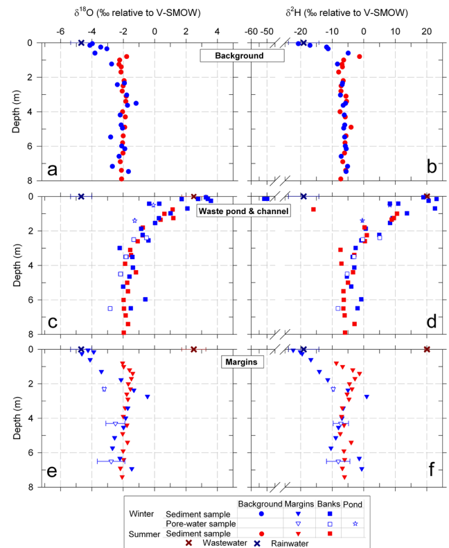
Fig. 4. \delta^{18}\text{O} and \delta^2\text{H} in rainwater, wastewater, pore water and in undisturbed sediment samples from the vadose zone underlying the undisturbed background site (a, b), permanently flooded waste pond and channel (c, d) and waste source margins (e, f). The top sample represents an average value for the 0–1.2 m depth, section. Values for the depths of 0–0.3 m were obtained only at the end of the winter, from sediment samples taken by a garden hand shovel.
