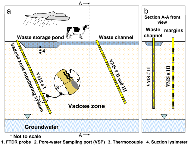
Fig. 3. Schematic side-view illustration of the vadose-zone monitoring system (VMS) installed under the waste storage pond, waste channel and the waste channel margins (a), and front view (A-A) of the VMS installed under the channel and its margins (b) (modified from Baram et al., 2012a).
