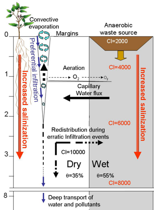
Fig. 8. Desiccation-crack-induced-salinization (DCIS) conceptual model.
