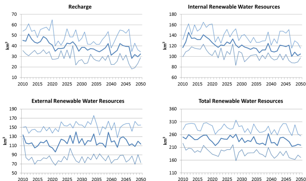
Fig. 7. Total gross recharge, internal, external and total renewable water resources from 2010 to 2050. The thick line is the average of the nine GCMs, and the thin lines show the second wettest and second driest GCM.
