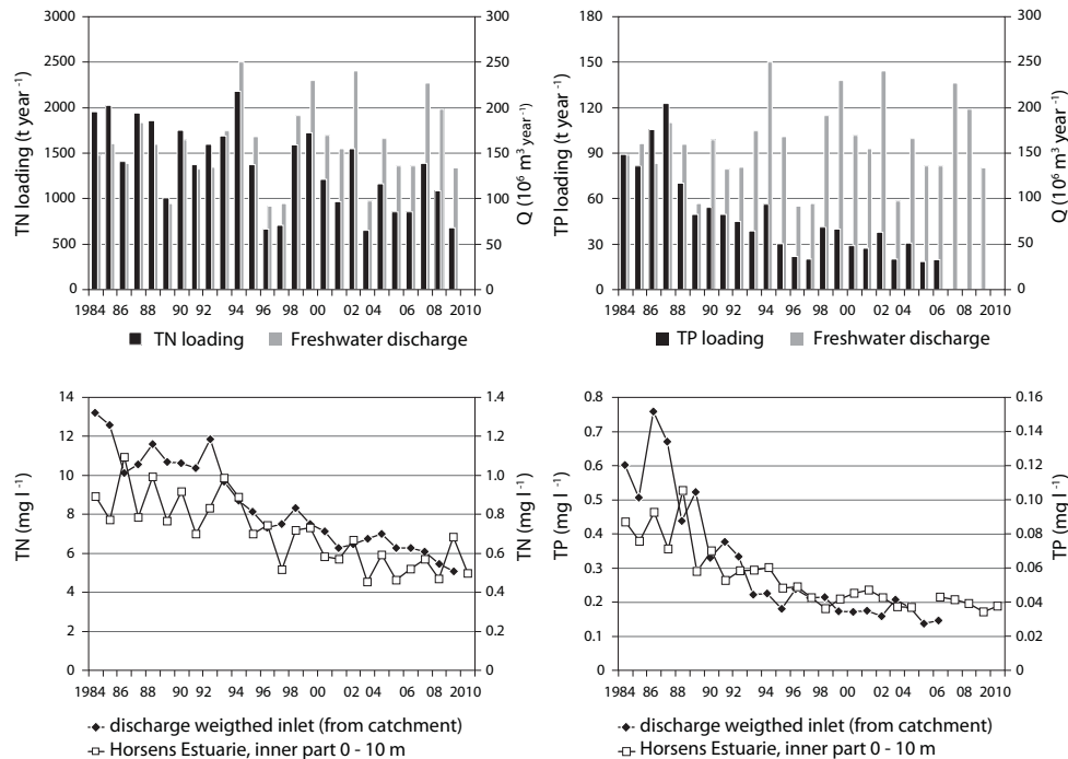
Fig. 4. Historical development of freshwater discharge and TN and TP loadings to Horsens estuary (upper figures), discharge weighted concentrations in the freshwater inlet to the estuary and annual average concentrations (0–10 m) in the inner part of the estuary (lower figures), 1984–2010.
