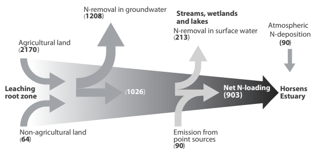
Fig. 5. Modeled nitrogen fluxes in the catchment of Horsens estuary and the net loading to the estuary, showing annual averages for the baseline period 2000–2005. Numbers in parenthesis are t N.
