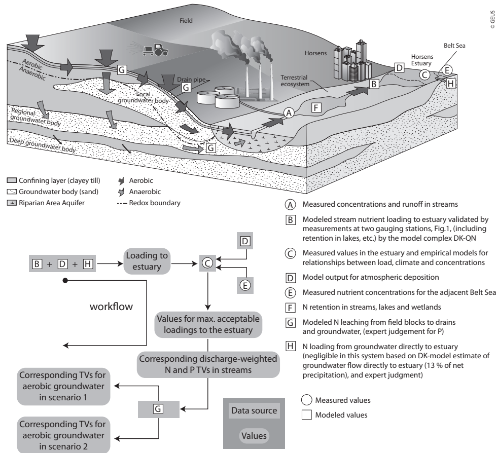
Fig. 2. Conceptual model of the catchment of Horsens estuary with indication of data and nutrient sources. The work process in calculation of threshold values (TVs) for streams and groundwater is indicated. The “DK-QN” model complex (or NLES & DK-QN & DK-model complex) is a combination of an empirical N leaching model (NLES, Kronvang et al., 2009b), an empirical monthly flow-weighted N concentration model from diffuse sources (DK-QN, Windolf et al., 2011), and a physically distributed integrated hydrological model (DK-model, Henriksen et al., 2003).
