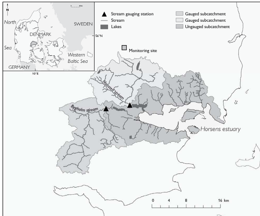
Fig. 1. Location and delineation of the investigated estuary and catchment, including stream gauging stations (triangles) and national monitoring site below farm land (square).
