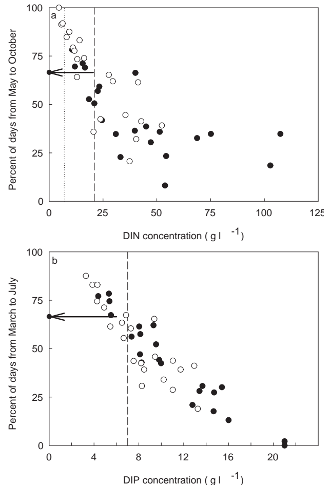
Fig. 8. (a) Relationship between mean concentration and percent of days with limitation for inorganic nitrogen, DIN, and (b) inorganic phosphorous, DIP. Calculated annually from 1985 to 2006 for Horsens estuary; filled circles (inner part), open circles (outer part), respectively. For DIN the calculations are performed on data from May to October (184 days), and limitation is assumed to occur when \text{DIN} < 14 \mu\text{g l}^{-1} . For DIP the period is from March to July (153 days), and limitation is assumed to occur when \text{DIP} < 6.2 \mu\text{g l}^{-1} . The vertical dashed lines indicate when limitations occur for 2/3 of the time, and the corresponding concentrations ( \text{DIN } 21 \mu\text{g l}^{-1} , \text{DIP } 7 \mu\text{g l}^{-1} ) are considered the target values for good ecological status of the estuary. The vertical dotted line is the resulting DIN concentration for the outer part of the estuary with an annual N load of 560 \text{ t yr}^{-1} .
