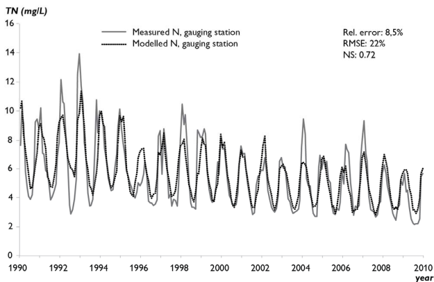
Fig. 3. Measured and simulated TN concentrations at the gauging station on Hansted stream (see Fig. 1).
