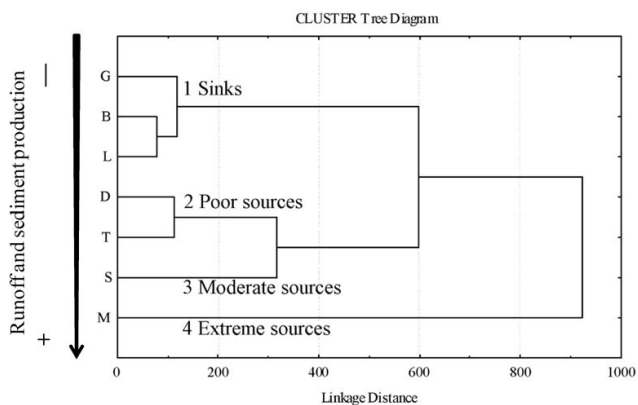
Fig. 5. Dendrogram of the cluster classification analysis with hydrological data of the different patches. G: Genista ; B: Brachypodium ; L: Lolium ; T: Thymus ; D: Dactylis ; S: Santolina ; M: Medicago .
