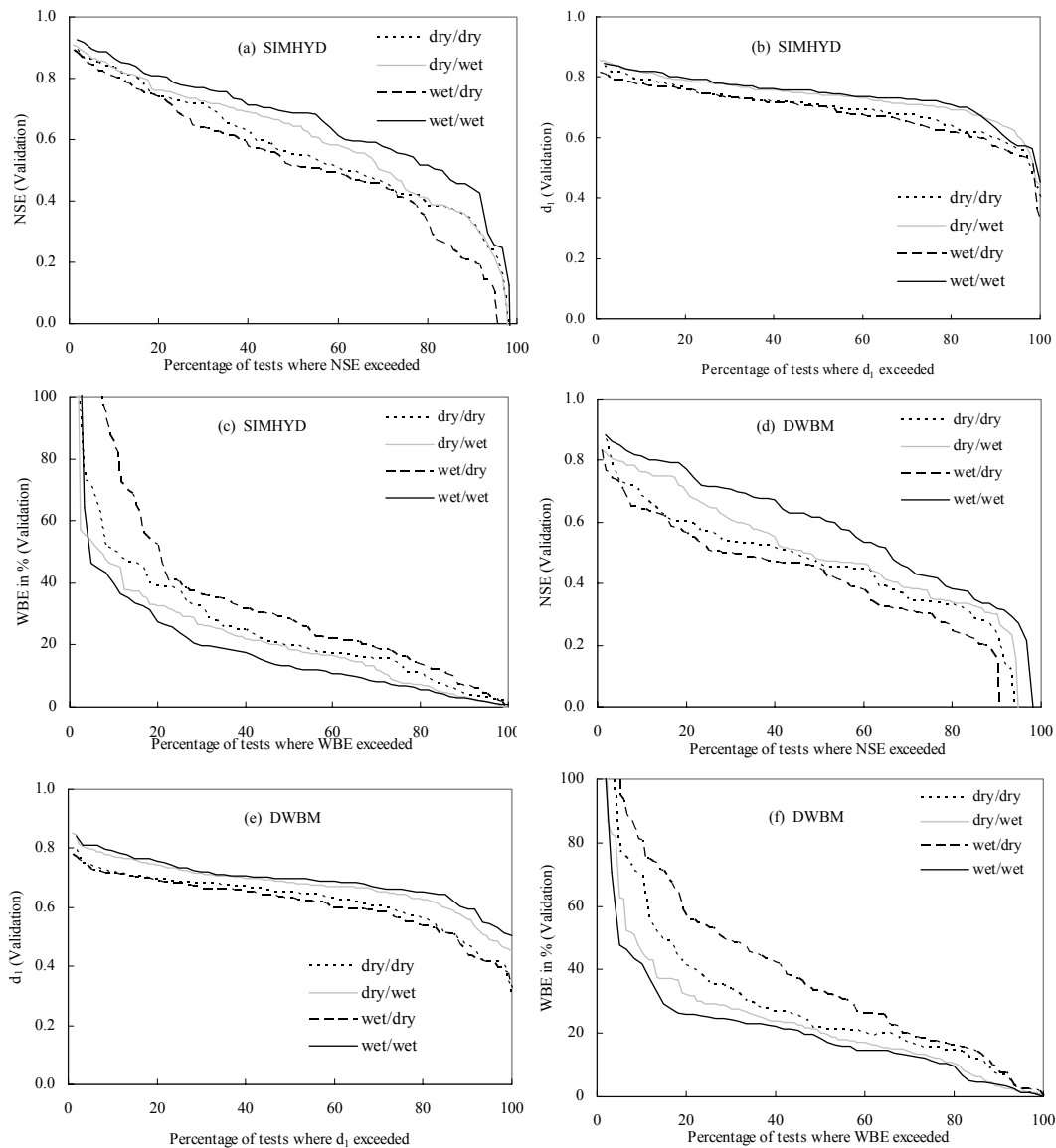
Fig. 6. Panels (a) and (d): percentage of model validation tests with a NSE value greater than or equal to a given NSE value. Similarly, panels (b) and (e), (c) and (f) are corresponding plots of the modified index of agreement ( d_1 ), the water balance error (WBE), respectively.
