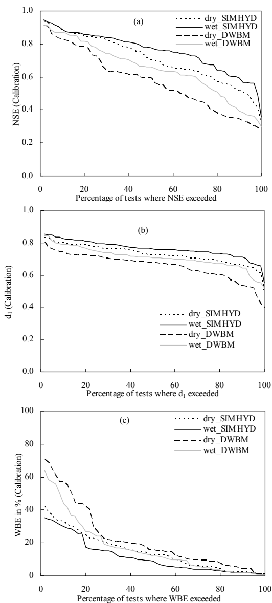
Fig. 5. (a) Percentage of model calibration tests with a NSE value greater than or equal to a given NSE value. Similarly, panels (b–c) are corresponding plots of the modified index of agreement ( d_1 ), the water balance error (WBE), respectively.
