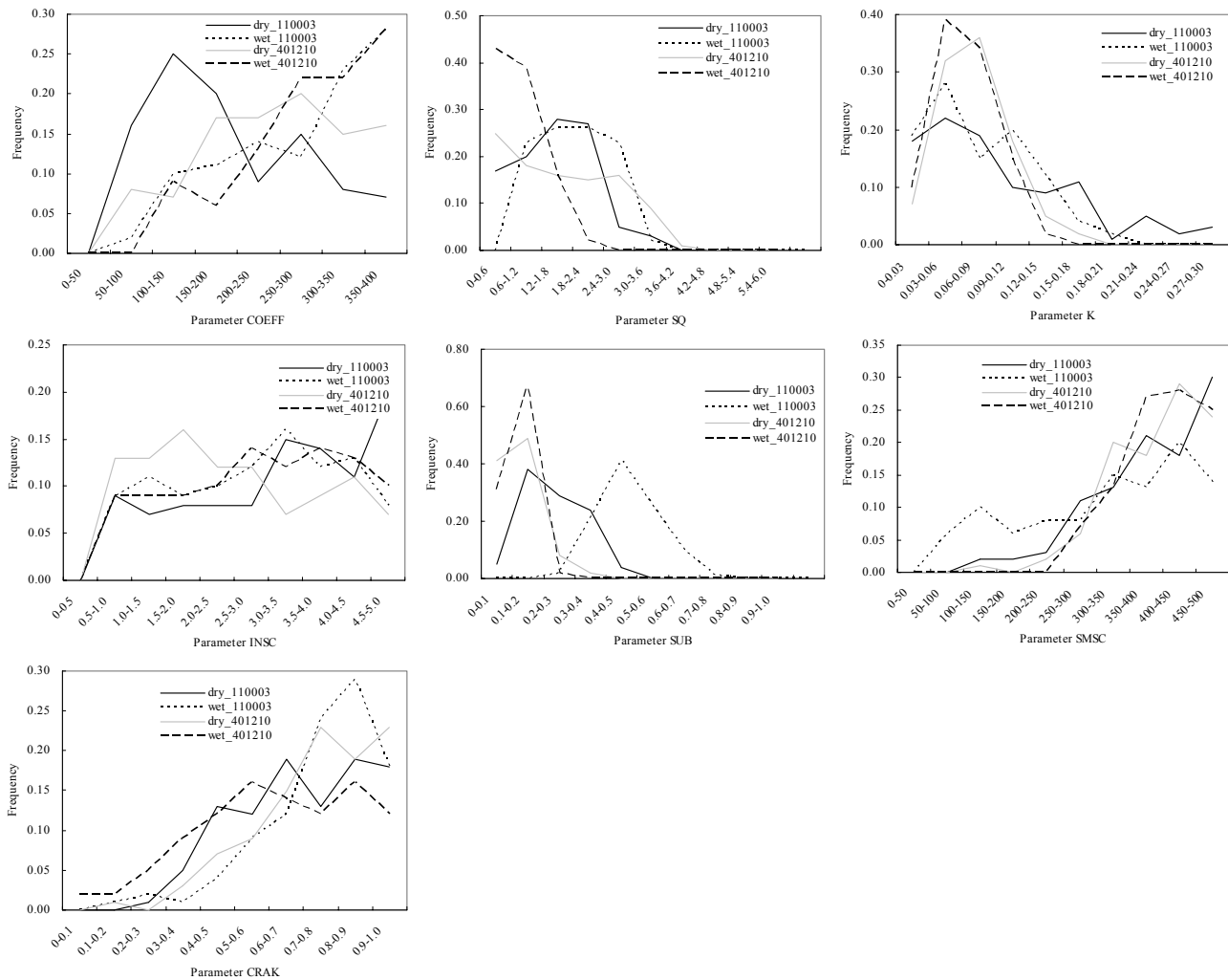
Fig. 7. Probability density functions for 7 parameters of the SIMHYD model under dry and wet calibration periods in catchments 110003 and 401210.
