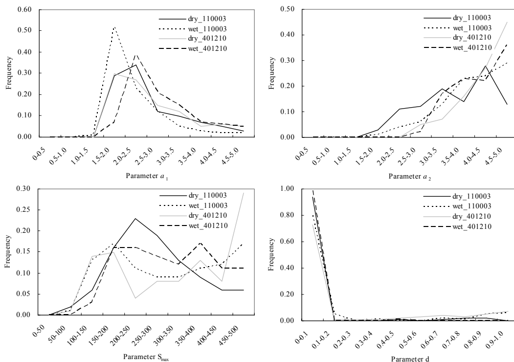
Fig. 8. Probability density functions for 4 parameters of the DWBM model under dry and wet calibration periods in catchments 110003 and 401210.
