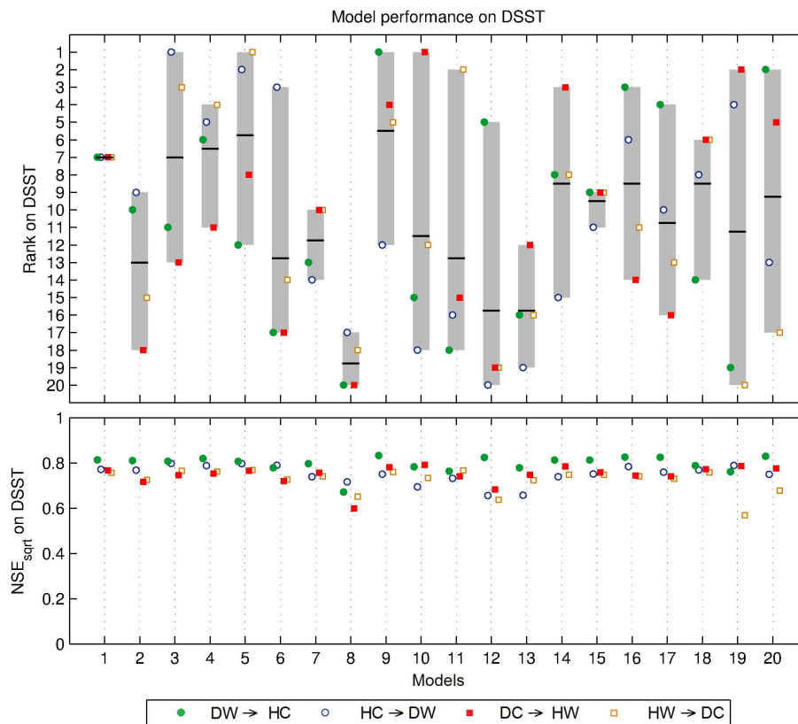
Fig. 6. Performance and rank in validation ( NSE_{\text{sqrt}} criterion) for the four DSST on the Au Saumon catchment (SAU).
