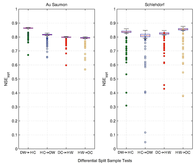
Fig. 13. Individual and multimodel DSST validation performance. Boxplots depict the range of the multimodel combinations, diamonds represent the twenty-model ensemble, and the circles and squares, the individual models, for the Au Saumon and Schlehdorf catchments.
