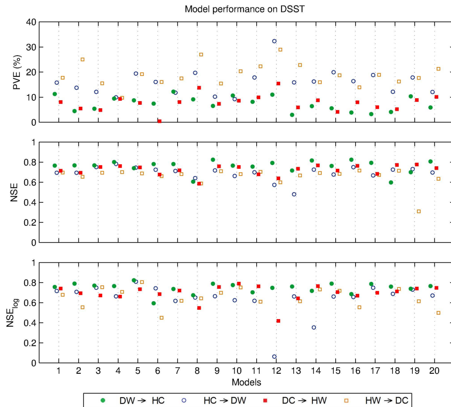
Fig. 7. Performance in validation (PVE, NSE and NSE_{\log} criterion) for the four DSST on the Au Saumon catchment (SAU). Negative values for NSE not shown.
