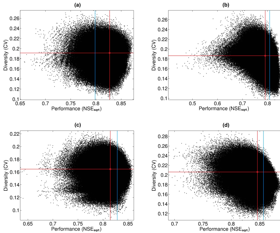
Fig. 12. Validation performance ( NSE_{sqrt} ) and diversity (CV) for all model combinations ( 2^{20} points) and Differential Split Sample Tests for the Schlehdorf catchment (SLD): (a) calibration on DW years (dry/warm) and validation on HC years (humid/cold); (b) calibration on HC years (humid/cold) and validation on DW years (dry/warm); (c) calibration on DC years (dry/cold) and validation on HW years (humid/warm); (d) calibration on HW years (humid/warm) and validation on DC years (dry/cold). Red lines and circle illustrate performance and diversity of the twenty-member ensembles and blue lines, of the best individual model for each test.
