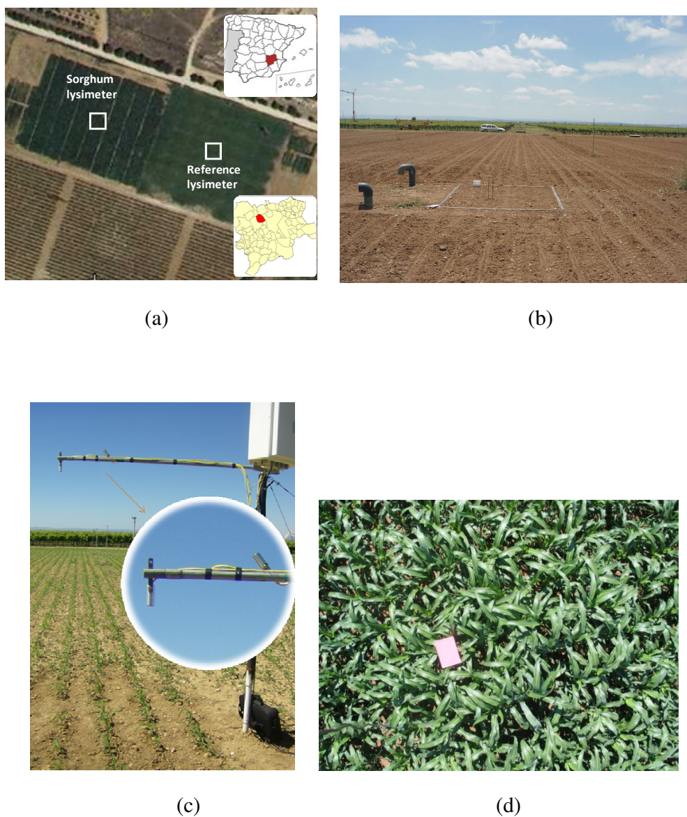
Fig. 1. (a) Location of the experimental site. (b) Lysimeter placed in the center of the sorghum field (picture from DOY 147). (c) Experimental assembly of the two Apogee IRTs over the incipient sorghum (picture from DOY 172). (d) Nadir view of the developed sorghum (picture from DOY 196).
