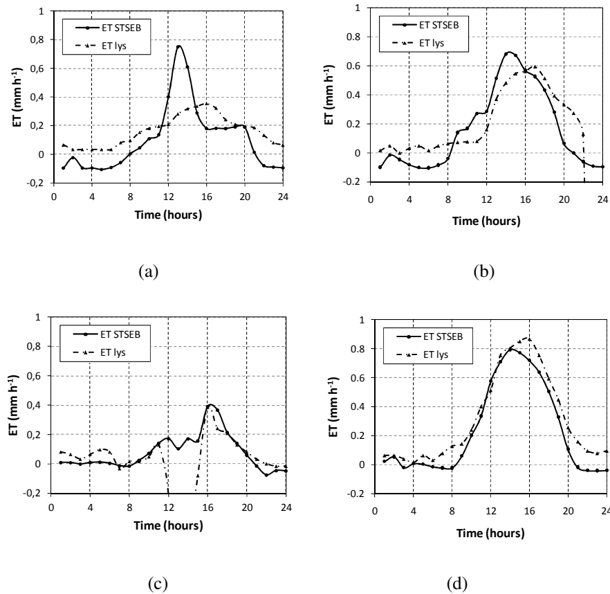
Fig. 5. Diurnal evolution of the estimated and measured sorghum ET: (a) DOY 184, (b) DOY 185, (c) DOY 229, (d) DOY 236.
