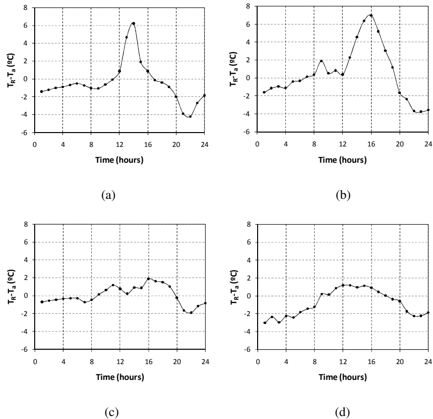
Fig. 3. Diurnal evolution of the gradient between sorghum radiometric temperature and air temperature: (a) DOY 184, (b) DOY 185, (c) DOY 229, (d) DOY 236.
