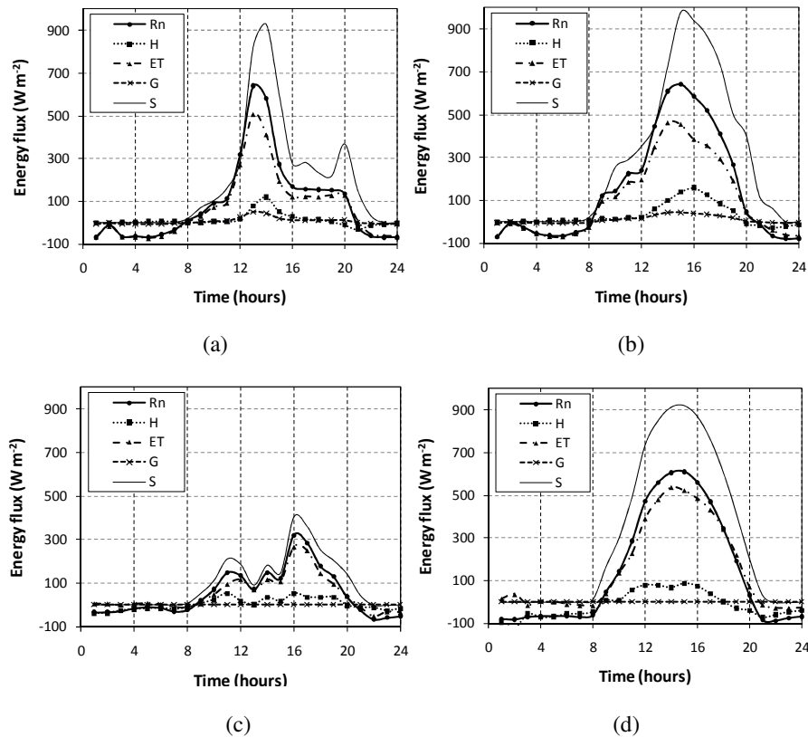
Fig. 4. Diurnal evolution of the sorghum flux components of the energy balance equation, together with the solar global radiation: (a) DOY 184, (b) DOY 185, (c) DOY 229, (d) DOY 236.
