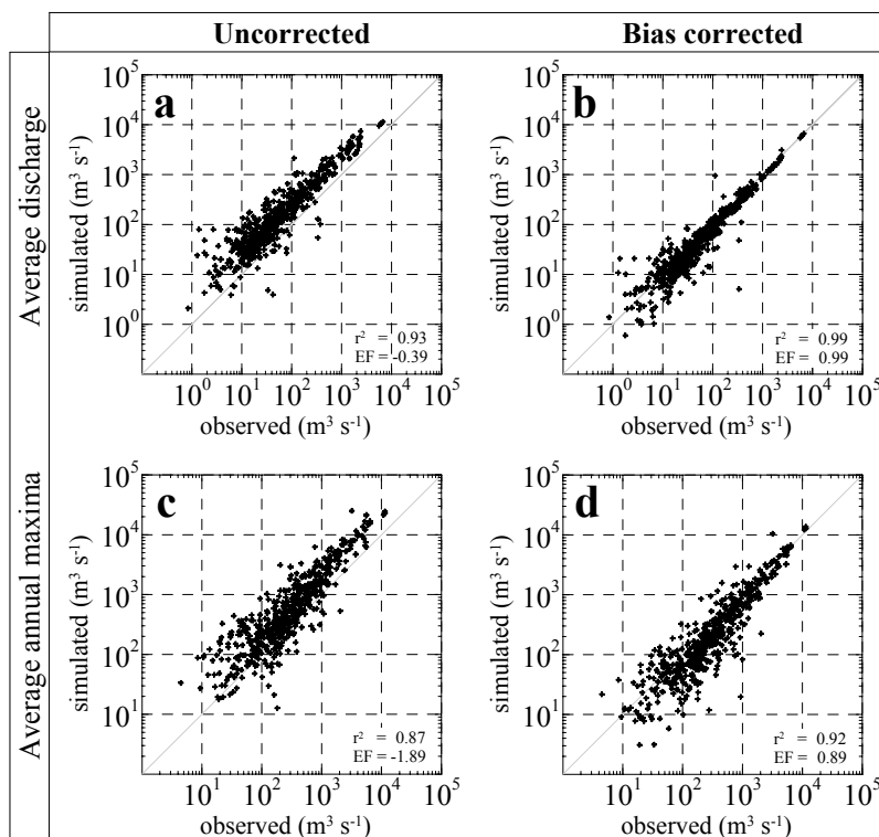
Fig. 10. Observed versus simulated average discharge (a, b) and average annual maximum discharge (c, d) for each of the 554 stations depicted in Fig. 1 for the control period 1961–1990. Left and right columns show hydrological simulations driven by uncorrected and bias corrected climate data, respectively.
