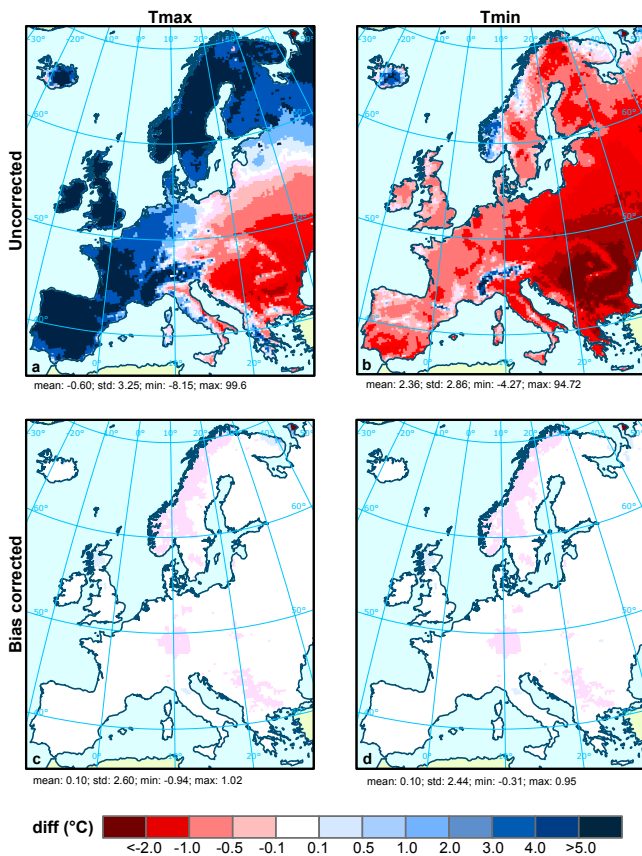
Fig. 7. Differences for daily maximum ( T_{max} ) and minimum ( T_{min} ) temperature simulated by HIRHAM5-ECHAM5 and the E-OBS data set for the control period 1961–1990. First row, uncorrected annual temperature; second row: bias corrected annual temperature.
