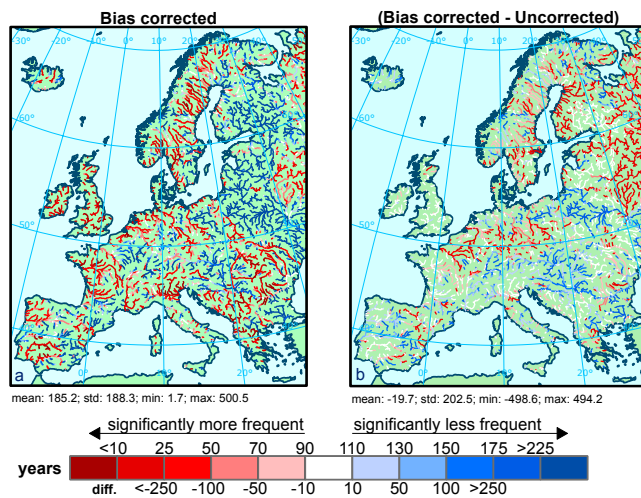
Fig. 13. (a) Recurrence interval of a 100-yr event observed in the control period (1961–1990) for the long-term future (2070–2099), and (b) difference (yr) for the recurrence interval of a 100-yr event between hydrological simulations driven by bias corrected and uncorrected climate data.
