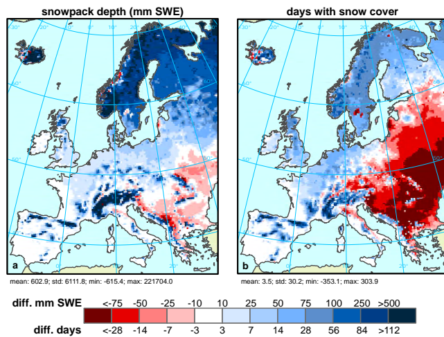
Fig. 9. Difference for LISFLOOD hydrological simulations driven by uncorrected and bias corrected climate data for the control period 1961–1990 for (a) snowpack depth (mm SWE) and (b) days with snow cover.
