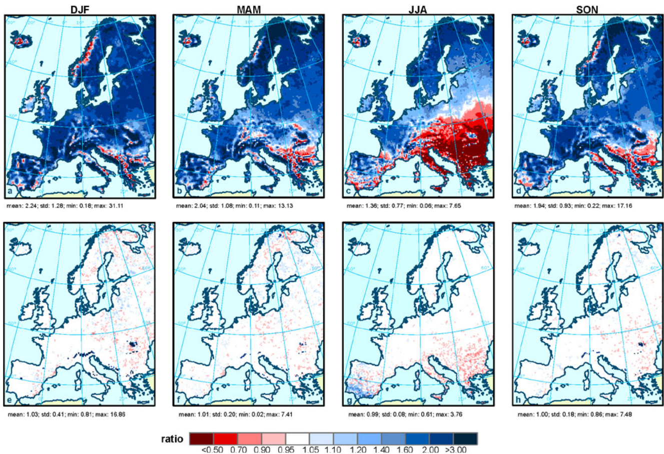
Fig. 2. Ratio between HIRHAM5-ECHAM5 simulations and observations of seasonal average precipitation for the control period 1961–1990. First row, uncorrected seasonal precipitation; second row, bias corrected seasonal precipitation.
