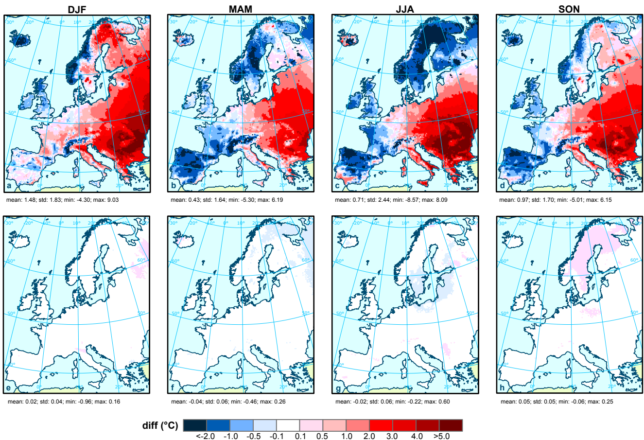
Fig. 6. Difference between HIRHAM5-ECHAM5 simulations and observations of seasonal average daily temperature for the period 1961–1990. First row, uncorrected seasonal temperature; second row: bias corrected seasonal temperature.
