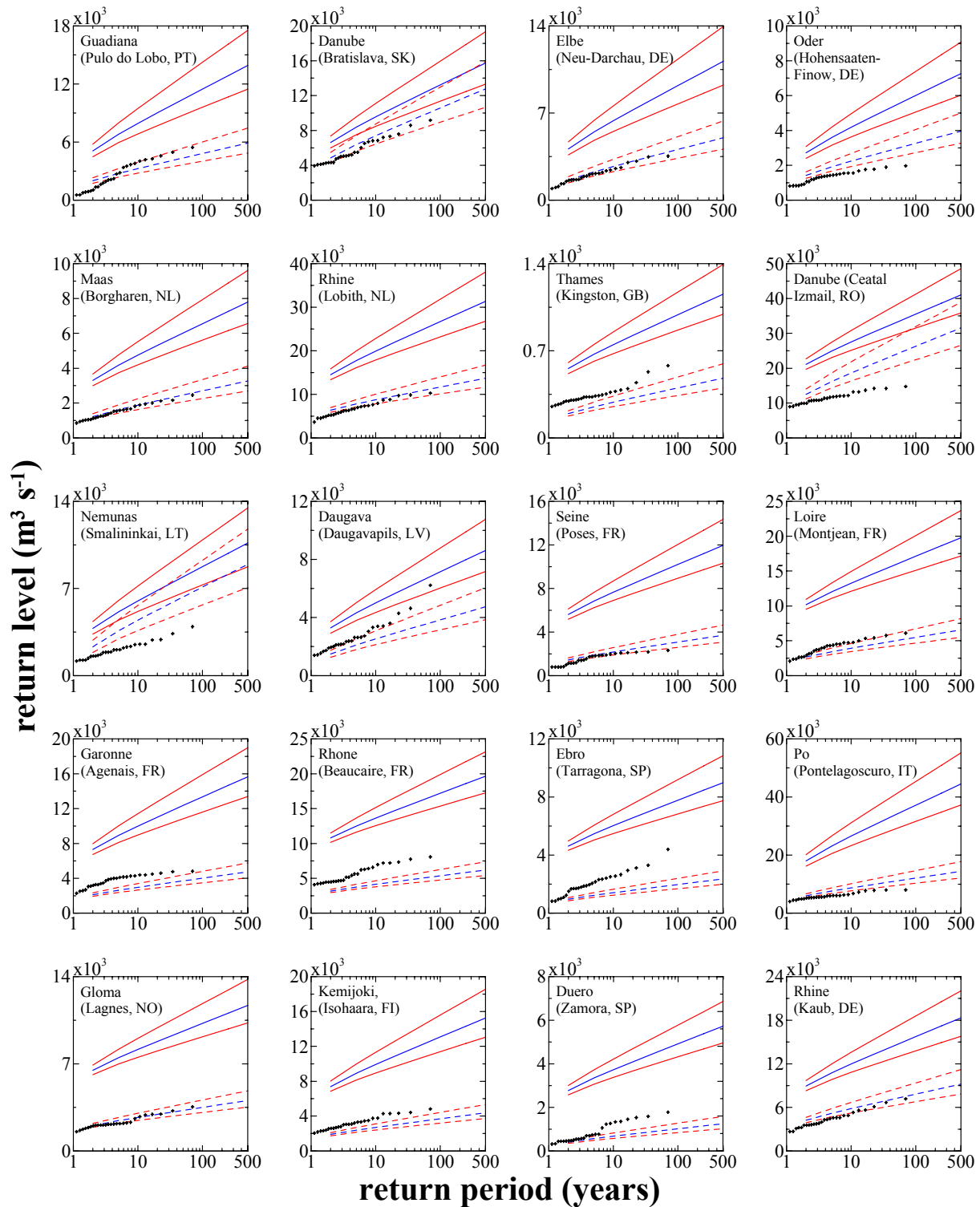
Fig. 11. Return level plots of simulated discharge levels in the 20 selected gauging stations showed in Fig. 1, based on a Gumbel distribution fit to the annual maxima for the control period 1961–1990. Full lines represent hydrological simulations driven by uncorrected forcing data whereas dashed lines represent the bias corrected counterpart. Also included in the plates are the 95 % confidence intervals (red dashed- and full-lines) derived using the profile-likelihood method. Black crosses represent return levels obtained from empirical plotting positions of observed annual maximum discharges at the selected stations.
