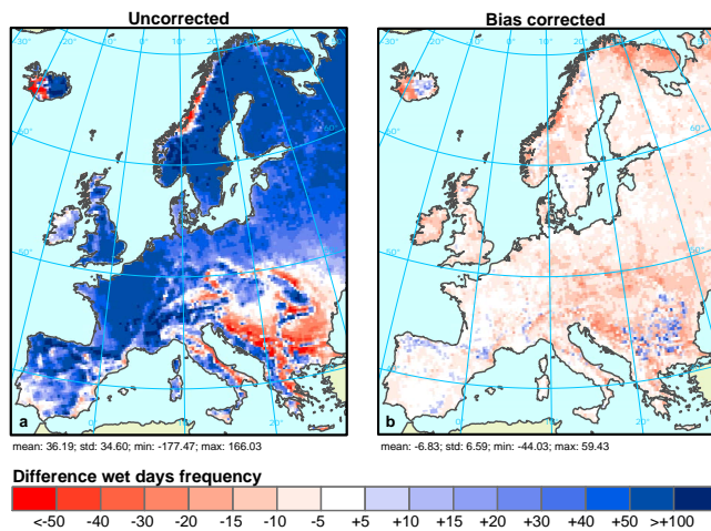
Fig. 3. Difference of average annual wet day frequency (precipitation \geq 1 \text{ mm d}^{-1} ) between (a) uncorrected precipitation and (b) bias corrected precipitation with respect to the E-OBS data set for the control period 1961–1990.
