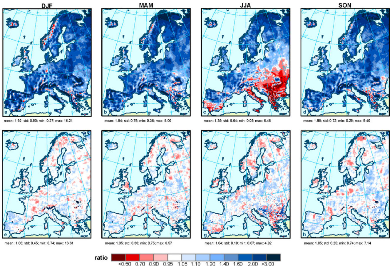
Fig. 4. Ratio between HIRHAM5-ECHAM5 simulations and observations of seasonal 99th percentile for the control period 1961–1990. First row, uncorrected seasonal precipitation; second row, bias corrected seasonal precipitation.
