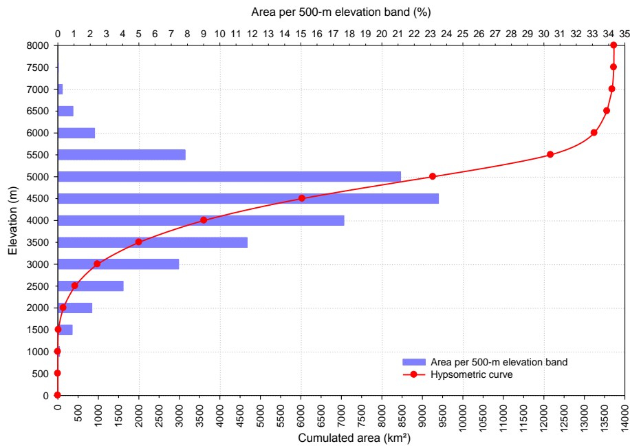
Fig. 3. Hypsometric curve of the Hunza River basin and distribution of the area by layer under each 500-m elevation band.
