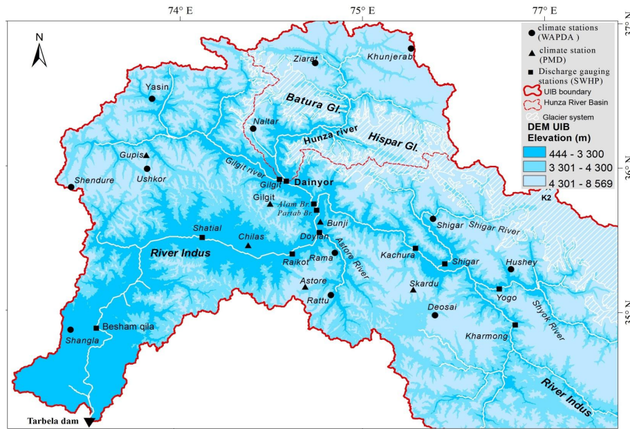
Fig. 2. ASTER Global digital elevation model (GDEM) of the Upper Indus River Basin and gauging station network within the boundary of Pakistan (Hunza River catchment location in the UIB is shown with a thin boundary line). The projection of the map is WGS1984 UTM 43N.
