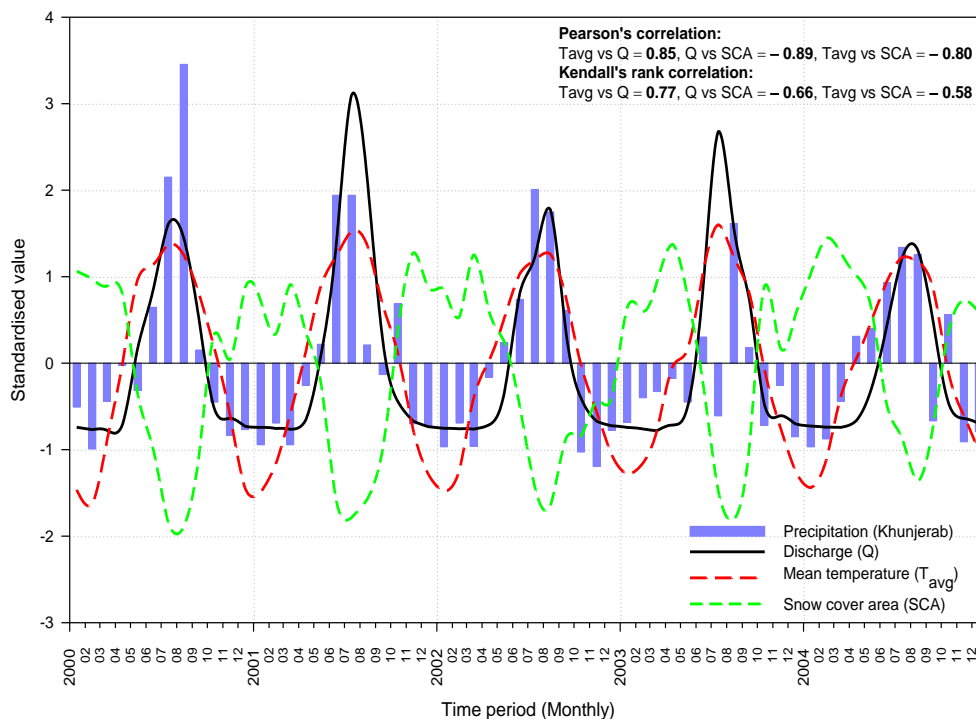
Fig. 7. Correlation between standardised values of precipitation (Khunjerab), snow cover, average temperature and discharge (at Dainyor) in the Hunza River basin (on a monthly basis). All the correlation values are significant with a significance level, p < 0.05 .
