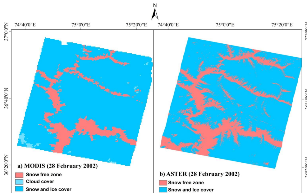
Fig. 4. (a) MODIS snow cover image and (b) ASTER snow cover image for the Hunza River basin. MODIS (MOD10A2) snow product is 8-day average data and the time span of this particular image presented here is from 25 February 2002 to 4 March 2002.
