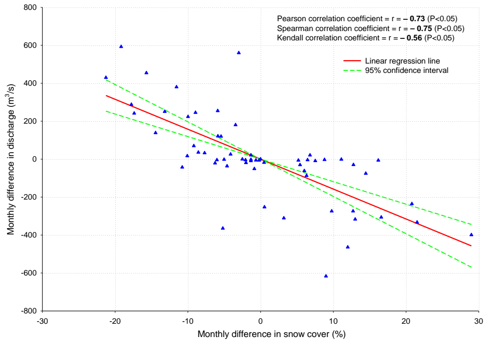
Fig. 8. Correlation between monthly difference in snow cover and monthly difference in discharge at Dainyor in the Hunza River basin. All the correlation values are significant with a significance level, p < 0.05 .
