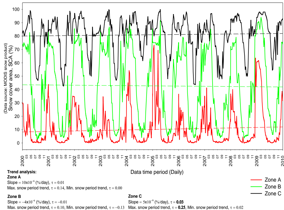
Fig. 5. Snow cover distribution in three different altitudinal zones of the Hunza River basin. Increasing trend (though not significant) can be noted in zone C. Seasonal Mann Kendall's trend analysis is also presented for maximum (November–February) and minimum (June–September) snow cover periods. (Kendall's tau ( \tau ) coefficient values presented in bold figures indicate an increasing trend with p < 0.05 ).
