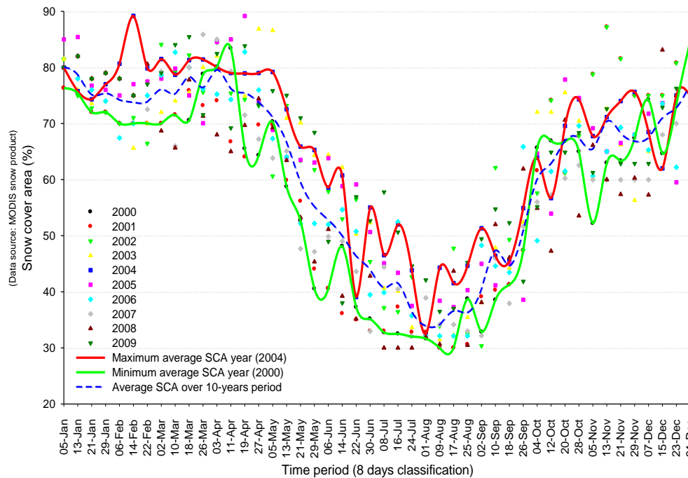
Fig. 6. Percentage snow cover area (SCA) in the Hunza River basin calculated by analysing 450 MODIS (MOD10A2) images.
