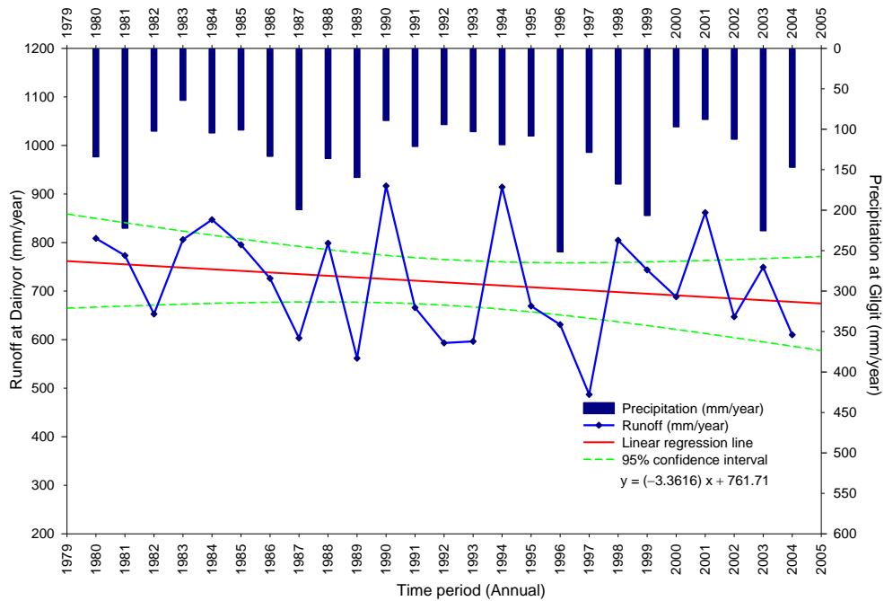
Fig. 9. Annual flow trend in Hunza River at Dainyor Bridge and total annual precipitation at Gilgit over 25 yr (1980–2004).
