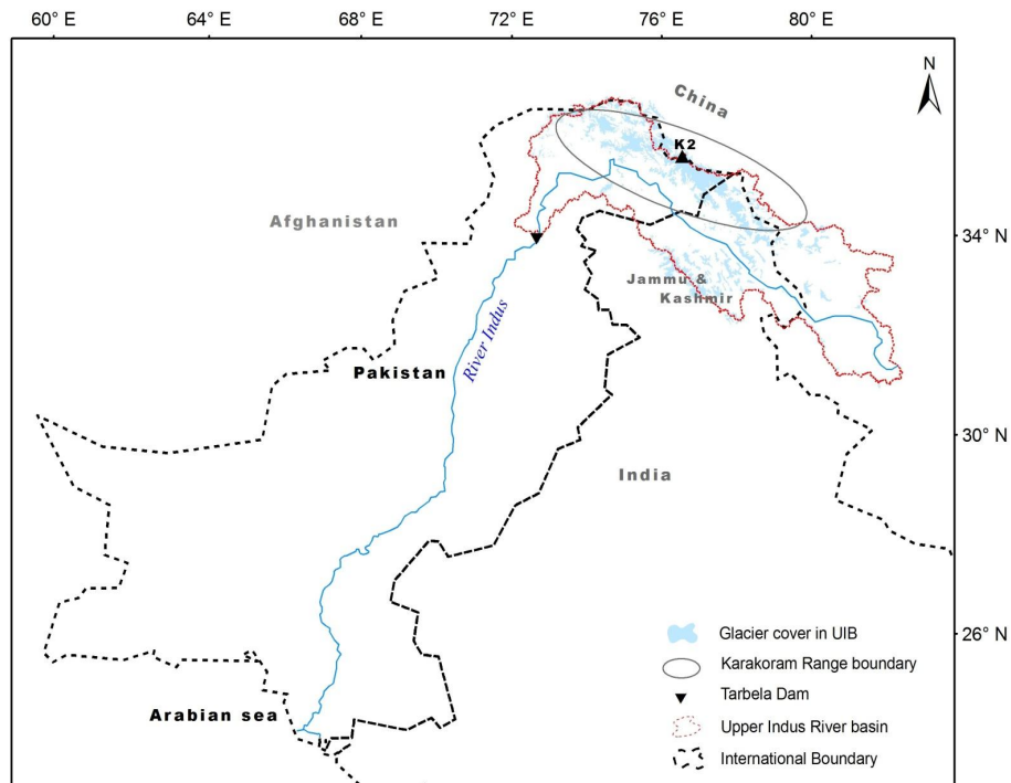
Fig. 1. Location of the Upper Indus River Basin (UIB) with main controlling storage at Tarbela Dam.
