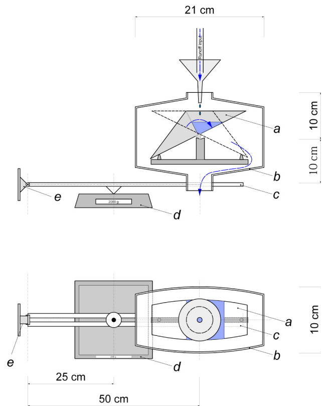
Fig. 2. Diagram of the weighable tipping bucket system. The blue arrow indicates the way the water has to go when leaving the (a) tipping bucket and (b) the box. The other parts of the set-up are (c) the lever connected to the balance by a screw, (d) the balance and (e) the pivot.
