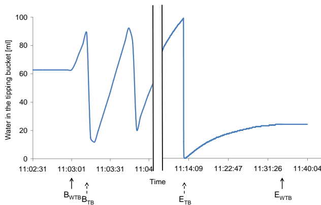
Fig. 4. Run-off event from concrete pavers at the 3rd of September 2009 in Berlin-Marienfelde. The dynamics were studied using the traditional tipping bucket (TB) signals compared to the weighable tipping bucket (WTB) data. B_{TB} , B_{WTB} and E_{TB} , E_{WTB} indicate the beginning and the end of the run-off event as detected by the tipping bucket and the weighable tipping bucket, respectively. Note, that the time axis is interrupted and scaled differently.
