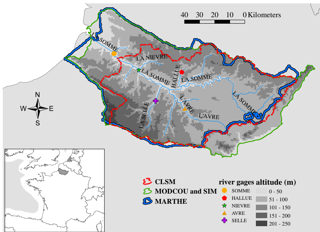
Fig. 1. Domains simulated by the four models: the domain used by CLSM corresponds to the surface topographic catchment upstream from Abbeville. MARTHE and MODCOU simulate a wider domain, as explained in the text. SIM uses the same domain as MODCOU.
