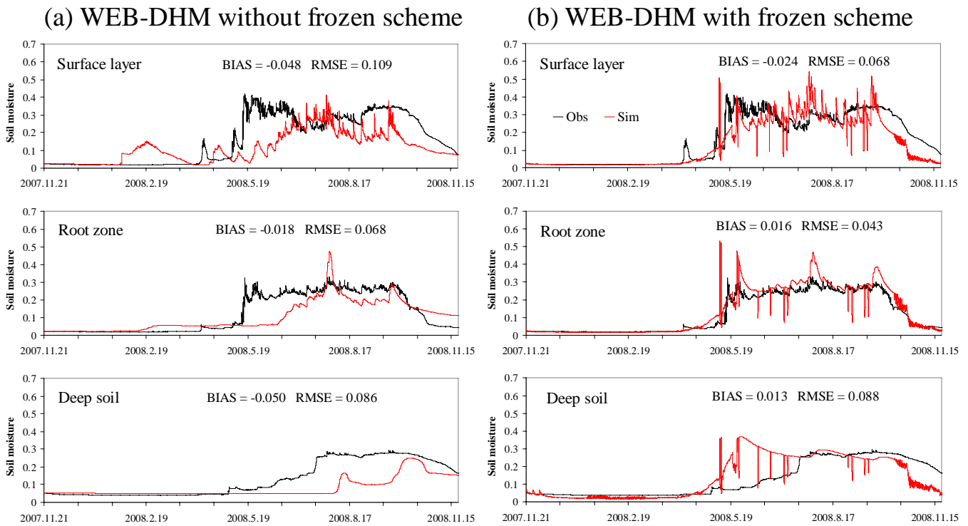
Fig. 10. Hourly volumetric liquid soil moisture averaged at surface layer (0–5 cm), root zone (5–25 cm), and deep soil layer (25–125 cm) at the DY station from 21 November 2007 to 20 November 2008, simulated by the WEB-DHM without and with the frozen scheme.
