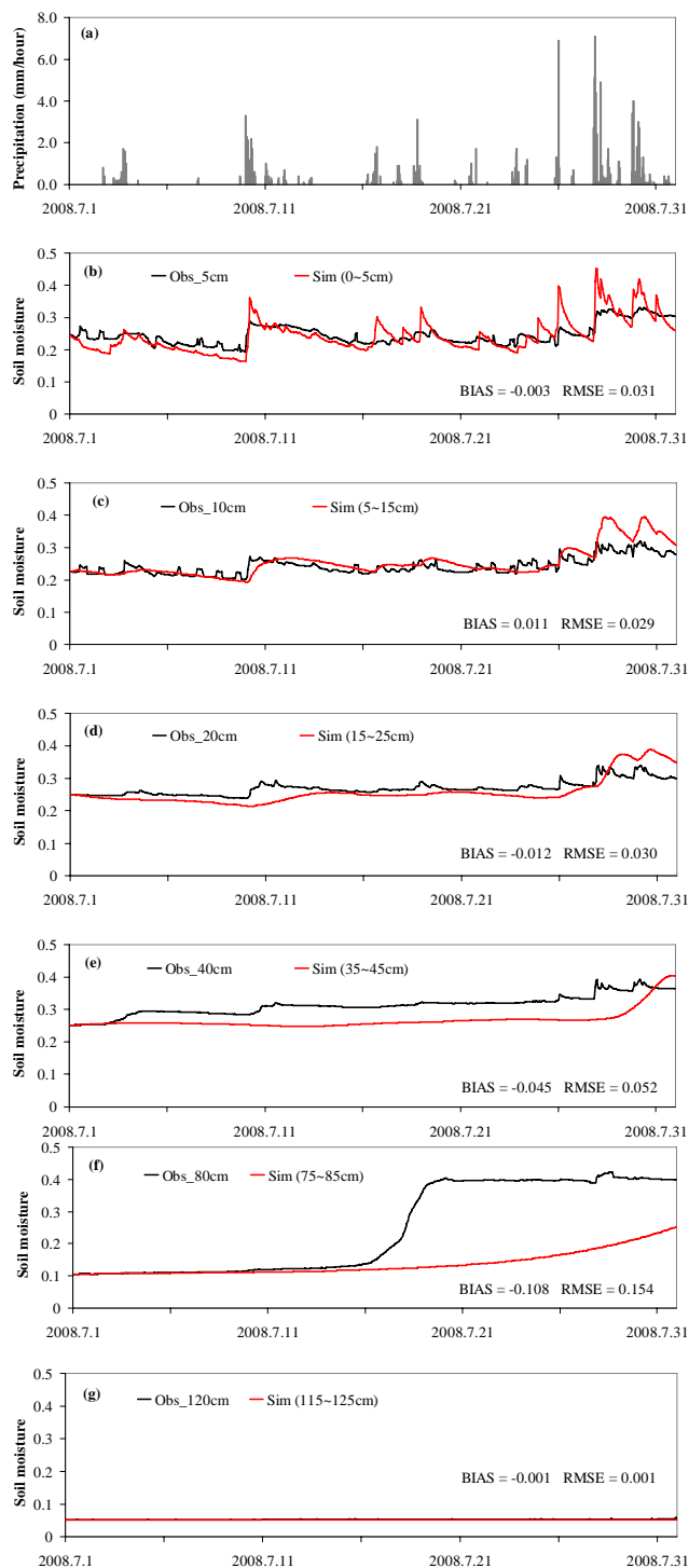
Fig. 5. Hourly precipitation (a), and the simulated and observed hourly volumetric liquid soil moisture at 5, 10, 20, 40, 80, and 120 cm (b–g) at the DY station in July 2008, by using the WEB-DHM without the frozen scheme.
