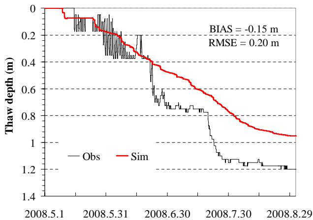
Fig. 7. Hourly observed (interpolated from the observations of soil temperature profile) and simulated thaw depth at the DY station, from 1 May to 31 August 2008, by using the WEB-DHM with the frozen scheme.
