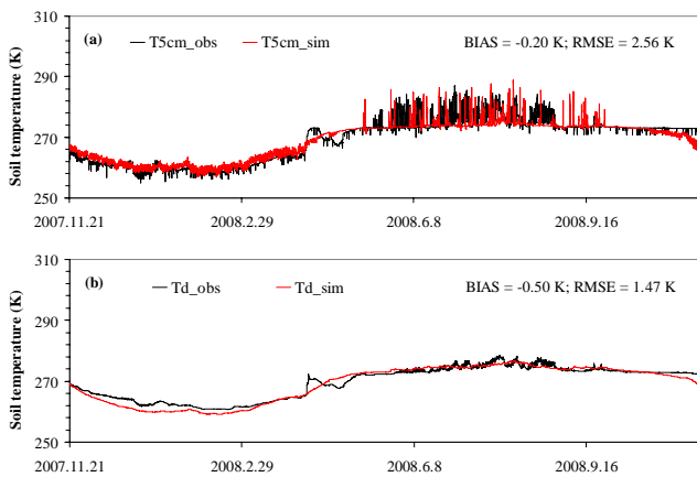
Fig. 8. Hourly observed and simulated temperature at 5 cm T_{5\text{cm}} (a) and temperature of deep soil T_d (b) at the DY station, from 21 November 2007 to 20 November 2008 by using the WEB-DHM with the frozen scheme.
