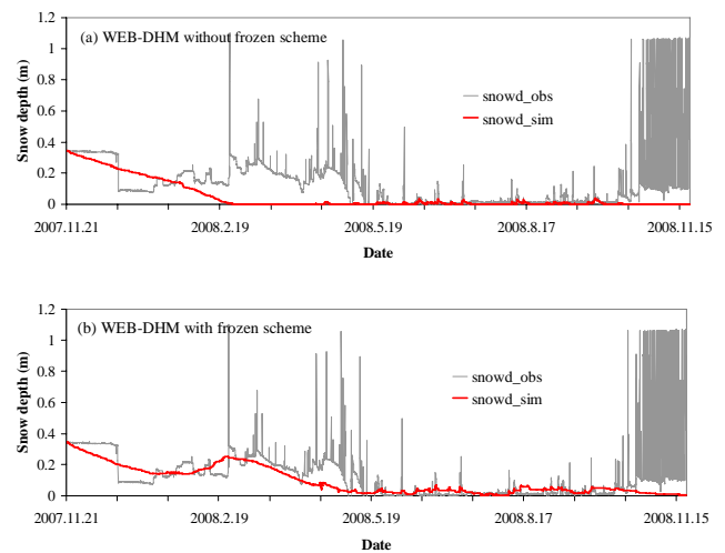
Fig. 9. Hourly snow depth at the DY station from 21 November 2007 to 20 November 2008, simulated by the WEB-DHM without and with the frozen scheme. Here, the snow depth is assumed as five times of the snow-water equivalent, and the large fluctuations of the observed snow depth at the station were caused by strong wind blowing.
