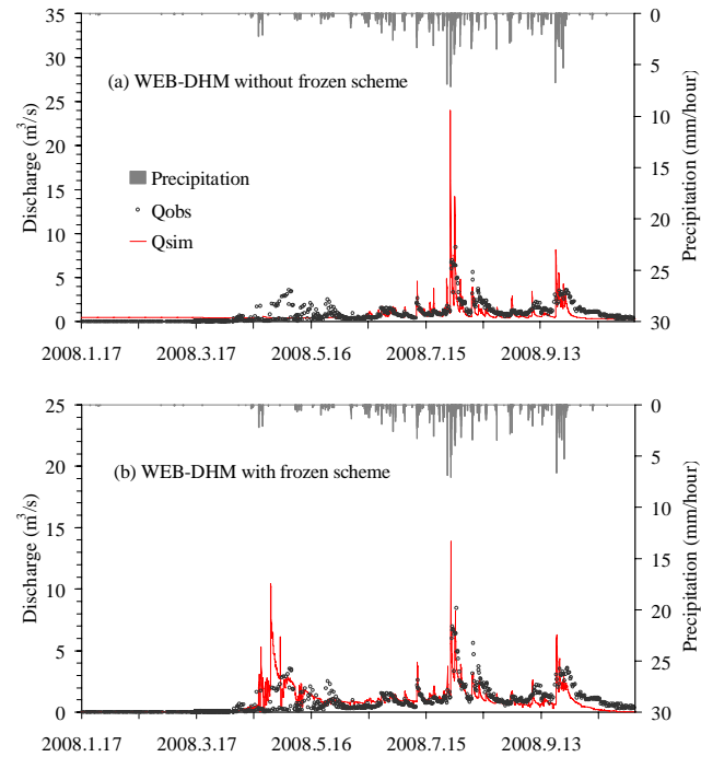
Fig. 11. Linear hourly hydrographs simulated by the WEB-DHM without and with the frozen scheme at the Binggou gauge from 17 January to 20 November 2008.
