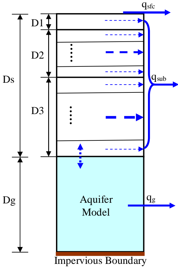
Fig. 2. Soil model of the WEB-DHM. Two different soil subdivision schemes are used for describing land surface and hydrological processes, respectively. The three-layer soil structure used in SiB2 is retained to represent the unsaturated zone in the calculations of land surface processes. The unsaturated zone is divided into multiple sublayers when simulating water flows within it and water exchanges with groundwater aquifer.
