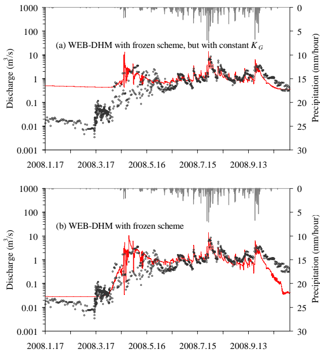
Fig. 12. Logarithmic hourly hydrographs simulated by using the WEB-DHM with the frozen scheme, neglecting (a) and considering (b) the frozen soil effect on the groundwater hydraulic conductivity at the Binggou gauge from 17 January to 20 November 2008.
