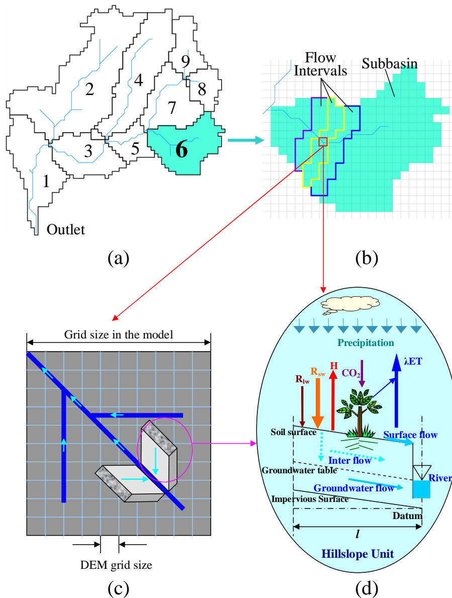
Fig. 1. Overall structure of WEB-DHM: (a) division from basin to sub-basins, (b) subdivision from sub-basin to flow intervals comprising several model grids, (c) discretization from a model grid to a number of geometrically symmetrical hillslopes, and (d) description of the water moisture transfer from atmosphere to river. Where R_{sw} and R_{lw} are downward solar radiation and longwave radiation, respectively, H is the sensible heat flux, and \lambda is the latent heat of vaporization. Here, the land surface submodel is used to describe the transfer of the turbulent fluxes (energy, water, and CO_2 ) between atmosphere and ground surface for each model grid; while the hydrological submodel simulates both surface and subsurface runoff using grid-hillslope discretization, and then simulates flow routing in the river network.
