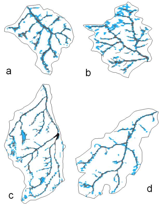
Fig. 4. Seasonal development of the spatial extent of the stream networks of Zastlerbach (a), Fichtenberger Rot (b), Haslach (c) and Eyach (d) with the reference (black line) and the simulated stream networks during spring (blue) and the late summer (dark grey).
