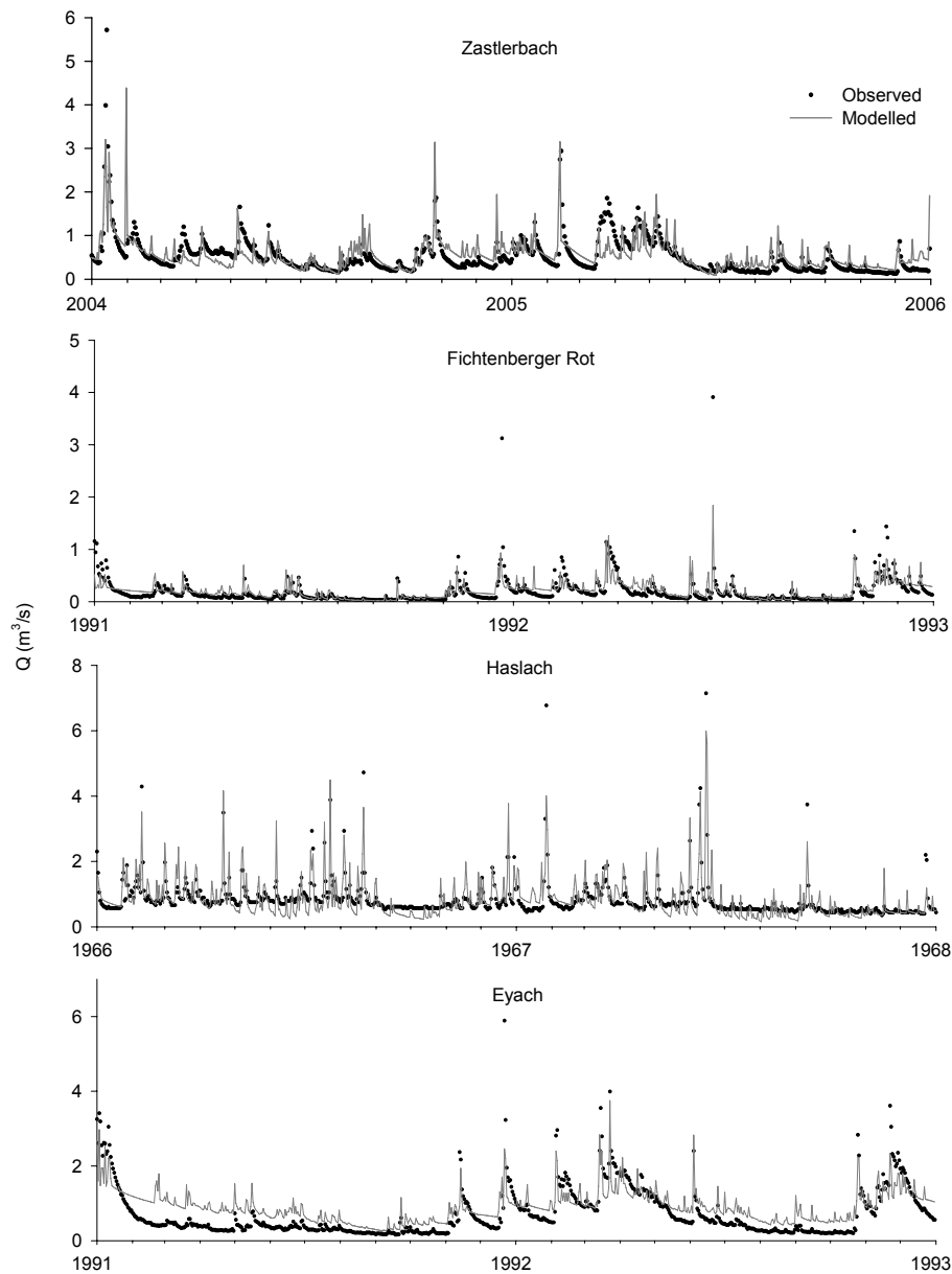
Fig. 5. Modelled and observed hydrographs of the four catchments.
