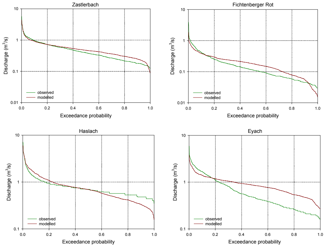
Fig. 6. Modelled and observed flow duration curves.
