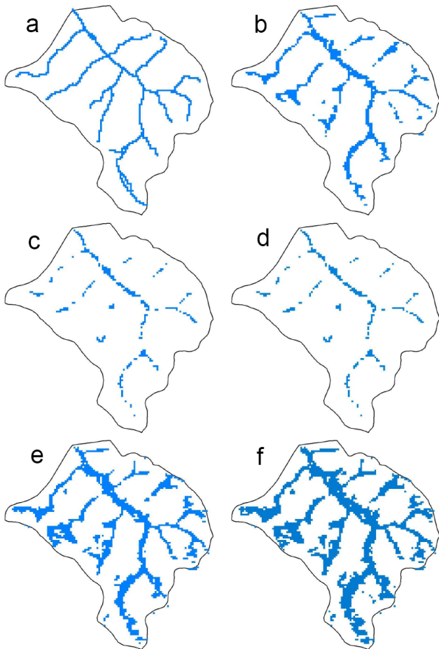
Fig. 3. Zastlerbach reference network (a) and effects of different parameter sets on the spatial distribution of stream cells (b–f).
