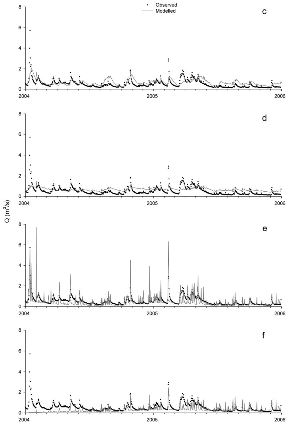
Fig. 7. Modelled and observed Zastlerbach hydrographs of the four test parameter sets specified in Table 5.
