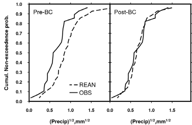
Fig. 4. CDFs for the same grid cell as in Fig. 3, but based on monthly average precipitation rate data for January for the “observed” period 1950–1976.
