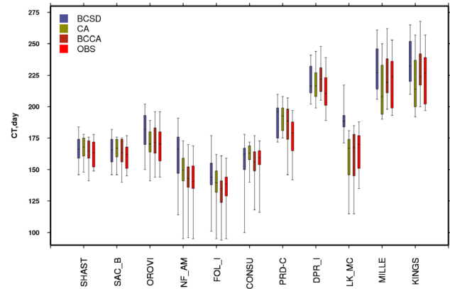
Fig. 5. Center timing for each streamflow site using each downscaling method, and the observationally-derived streamflows. Day is day of the water year, so 1 corresponds to 1 October.
